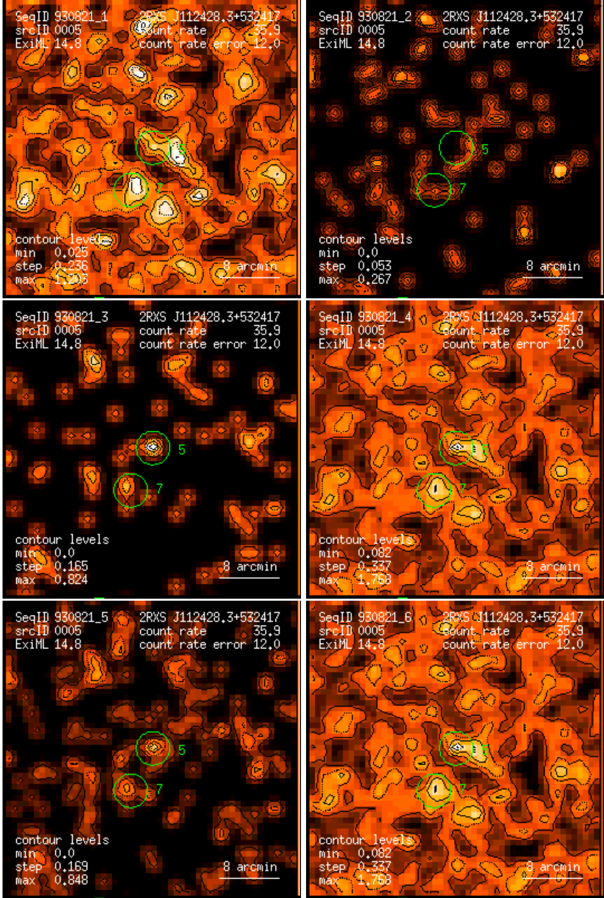
Figure 5: RASS 930821: detection 0005: band rate images, Gaussian filter: (1) PSPC channels 11 – 41, (2) 52 – 90, (3) 91 – 201, (4) 11 – 235, (5) 52 – 201, (6) 11 – 201. Broad band rates in counts/ks. Band rate contour levels in counts/ks/arcmin 2 .
