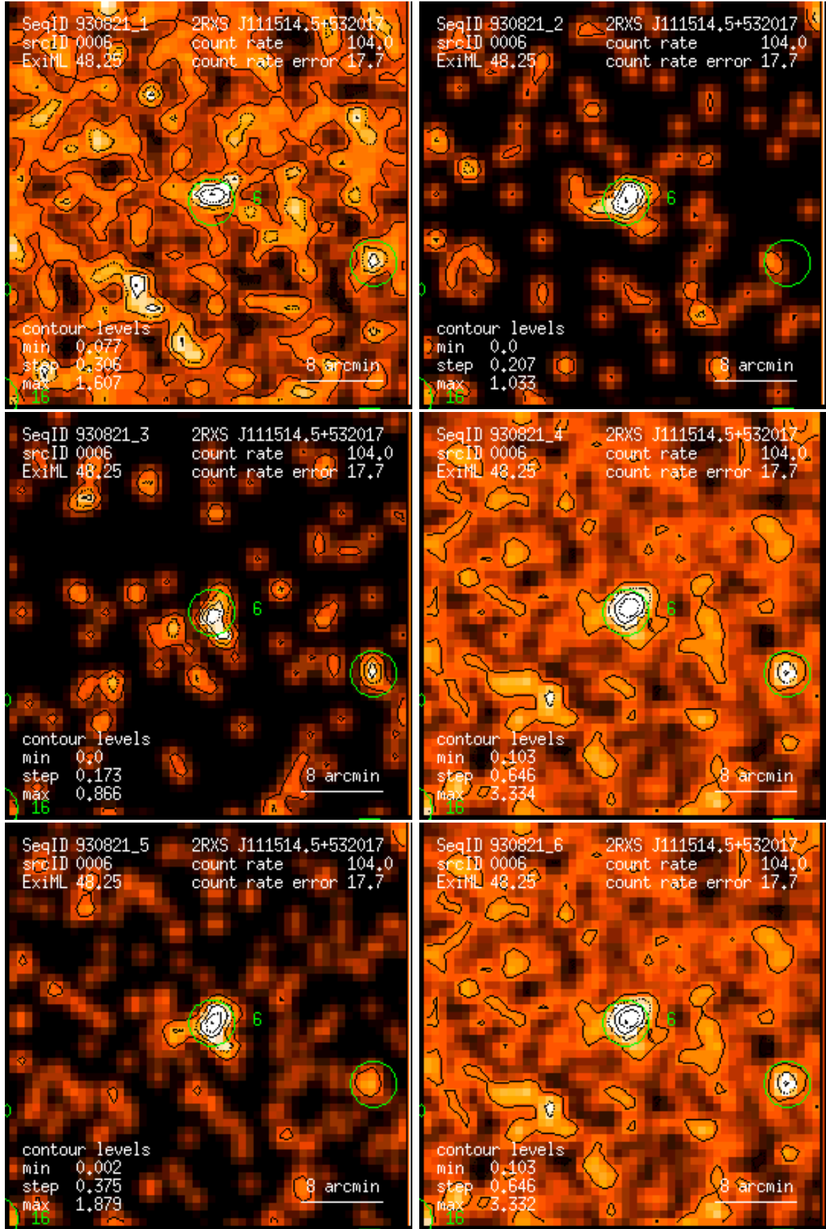
Figure 6: RASS 930821: detection 0006: band rate images, Gaussian filter: (1) PSPC channels 11 – 41, (2) 52 – 90, (3) 91 – 201, (4) 11 – 235, (5) 52 – 201, (6) 11 – 201. Broad band rates in counts/ks. Band rate contour levels in counts/ks/arcmin 2 .
