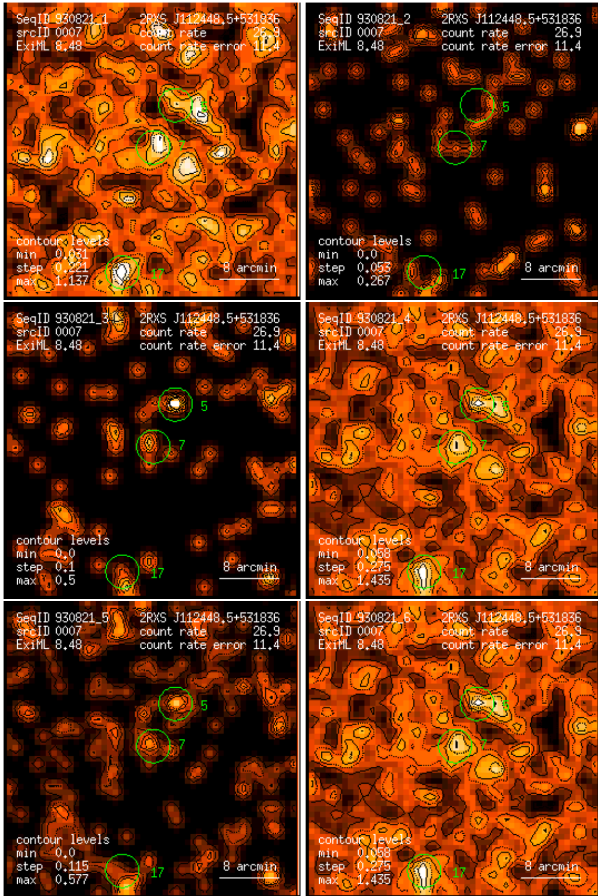
Figure 7: RASS 930821: detection 0007: band rate images, Gaussian filter: (1) PSPC channels 11 – 41, (2) 52 – 90, (3) 91 – 201, (4) 11 – 235, (5) 52 – 201, (6) 11 – 201. Broad band rates in counts/ks. Band rate contour levels in counts/ks/arcmin 2 .
