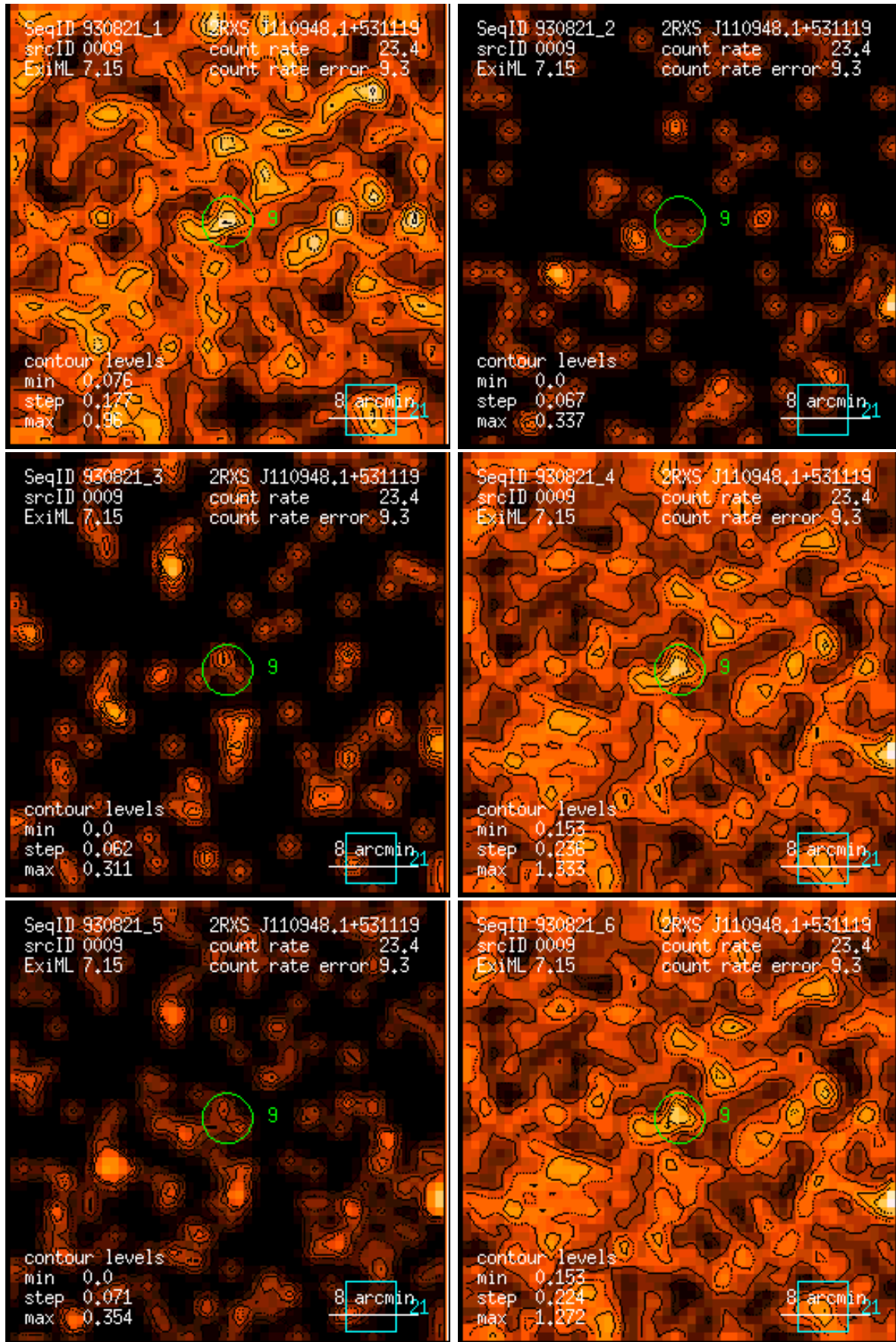
Figure 9: RASS 930821: detection 0009: band rate images, Gaussian filter: (1) PSPC channels 11 – 41, (2) 52 – 90, (3) 91 – 201, (4) 11 – 235, (5) 52 – 201, (6) 11 – 201. Broad band rates in counts/ks. Band rate contour levels in counts/ks/arcmin 2 .
