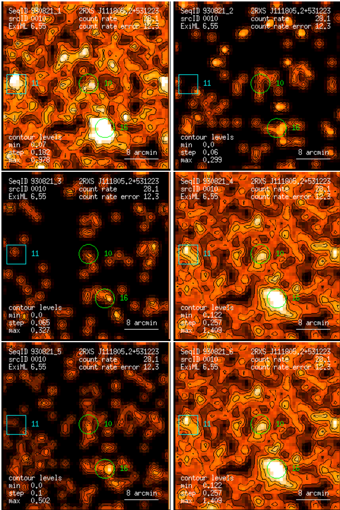
Figure 10: RASS 930821: detection 0010: band rate images, Gaussian filter: (1) PSPC channels 11 – 41, (2) 52 – 90, (3) 91 – 201, (4) 11 – 235, (5) 52 – 201, (6) 11 – 201. Broad band rates in counts/ks. Band rate contour levels in counts/ks/arcmin 2 .
