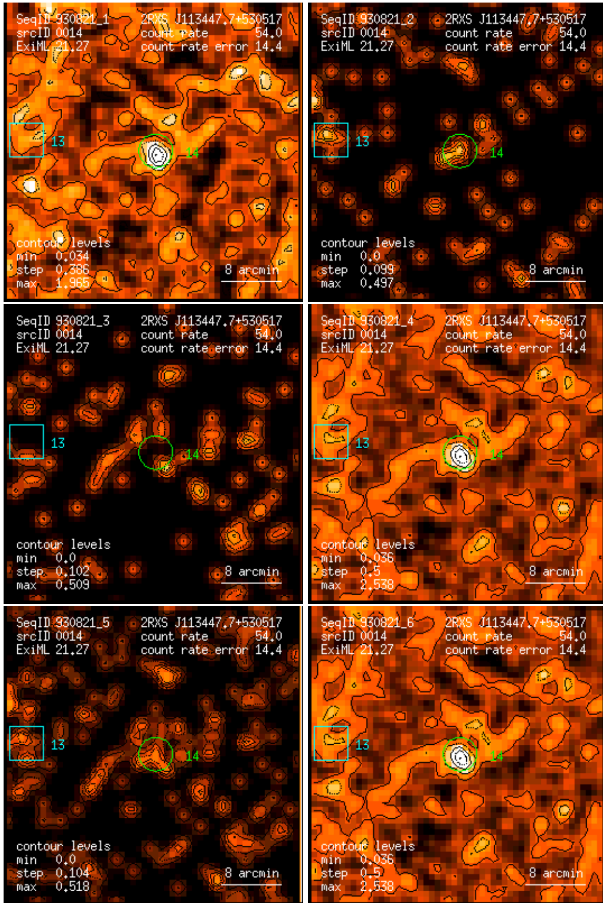
Figure 14: RASS 930821: detection 0014: band rate images, Gaussian filter: (1) PSPC channels 11 – 41, (2) 52 – 90, (3) 91 – 201, (4) 11 – 235, (5) 52 – 201, (6) 11 – 201. Broad band rates in counts/ks. Band rate contour levels in counts/ks/arcmin 2 .
