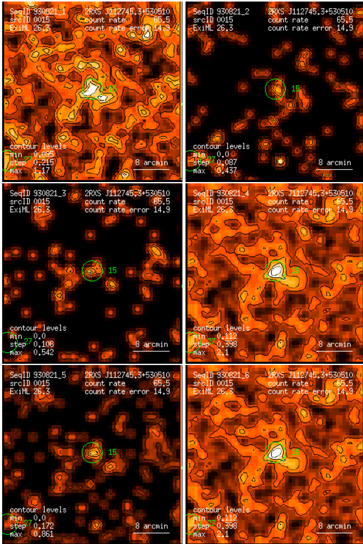
Figure 15: RASS 930821: detection 0015: band rate images, Gaussian filter: (1) PSPC channels 11 – 41, (2) 52 – 90, (3) 91 – 201, (4) 11 – 235, (5) 52 – 201, (6) 11 – 201. Broad band rates in counts/ks. Band rate contour levels in counts/ks/arcmin 2 .
