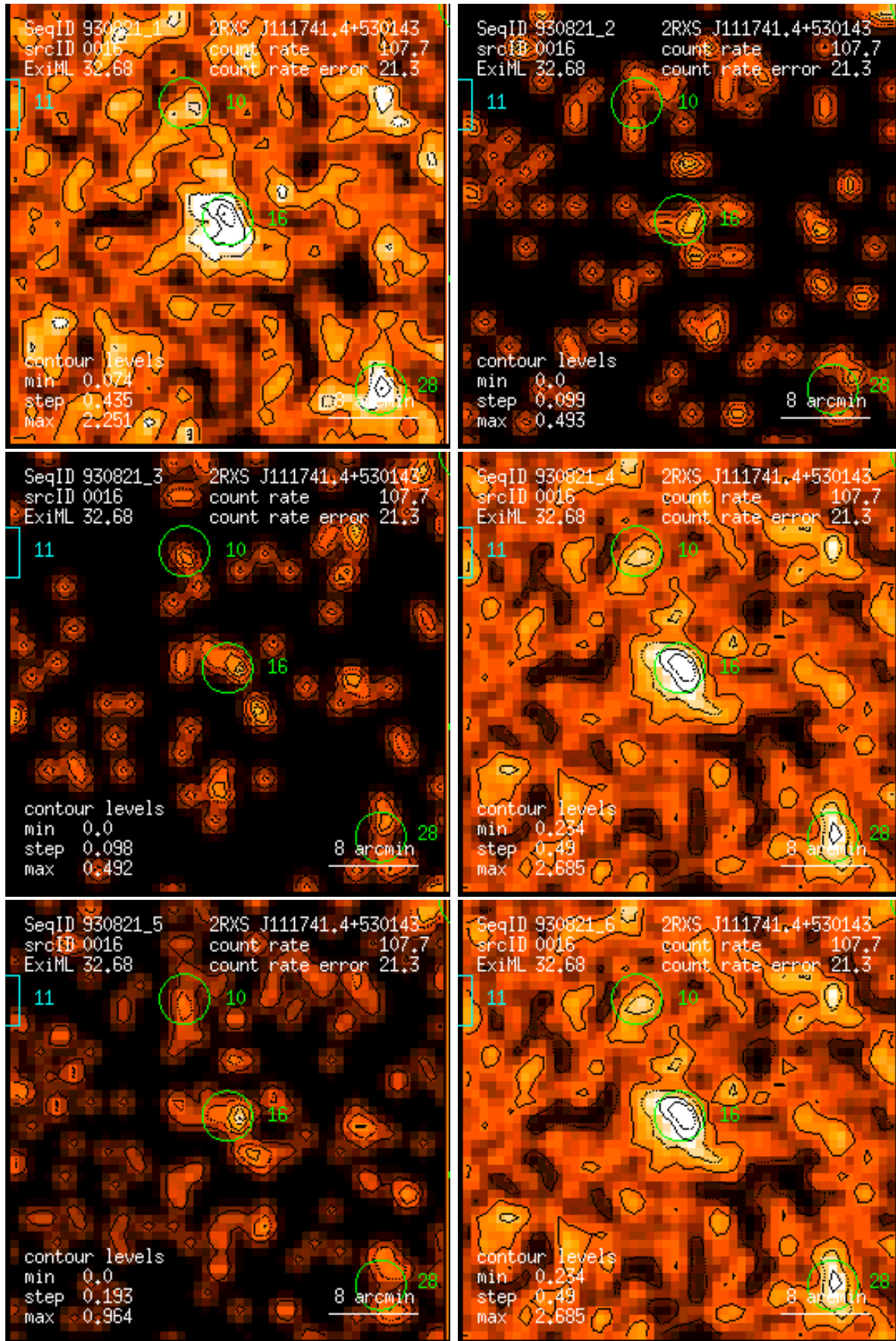
Figure 16: RASS 930821: detection 0016: band rate images, Gaussian filter: (1) PSPC channels 11 – 41, (2) 52 – 90, (3) 91 – 201, (4) 11 – 235, (5) 52 – 201, (6) 11 – 201. Broad band rates in counts/ks. Band rate contour levels in counts/ks/arcmin 2 .
