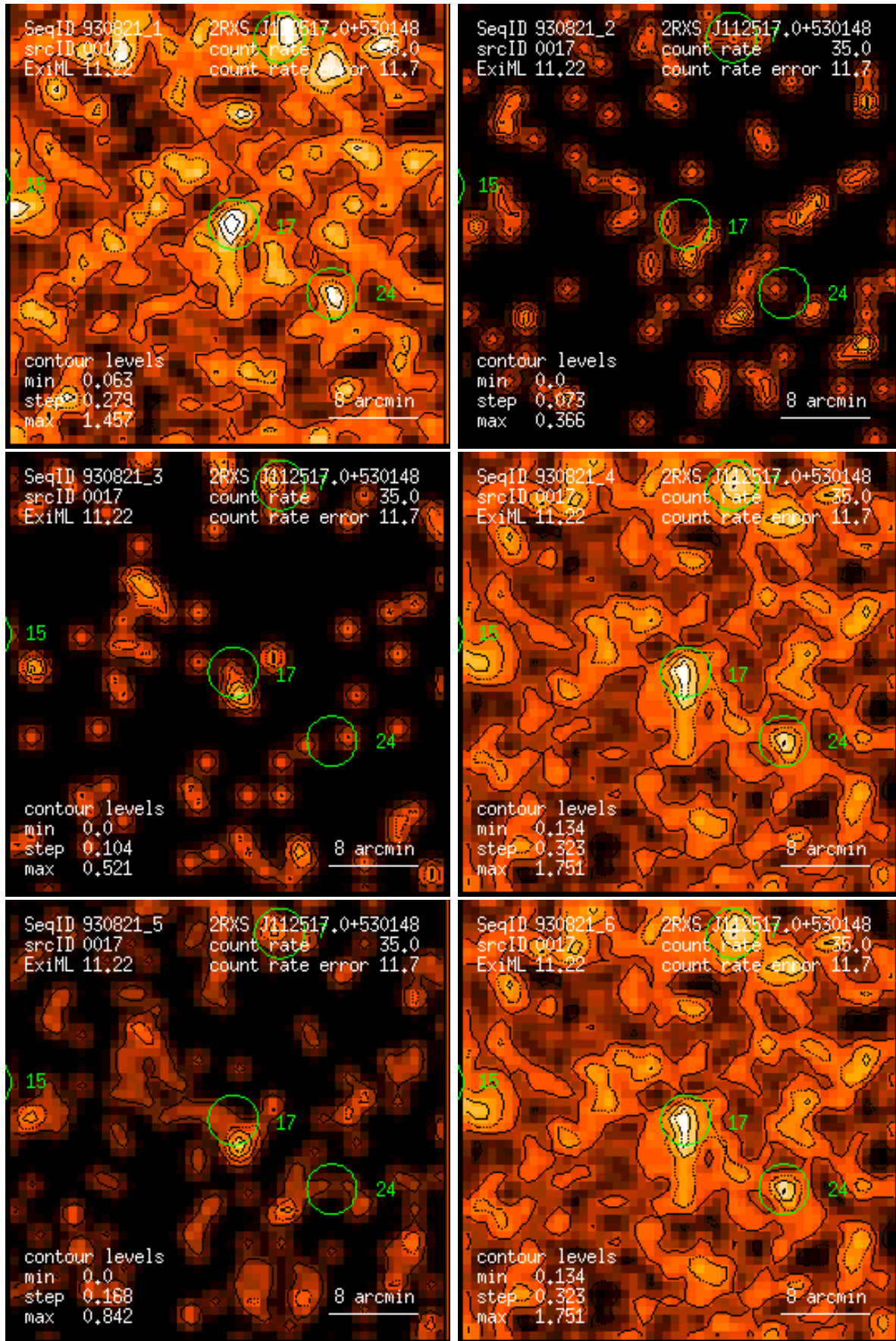
Figure 17: RASS 930821: detection 0017: band rate images, Gaussian filter: (1) PSPC channels 11 – 41, (2) 52 – 90, (3) 91 – 201, (4) 11 – 235, (5) 52 – 201, (6) 11 – 201. Broad band rates in counts/ks. Band rate contour levels in counts/ks/arcmin 2 .
