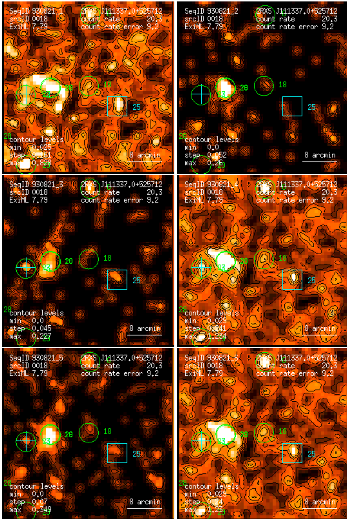
Figure 18: RASS 930821: detection 0018: band rate images, Gaussian filter: (1) PSPC channels 11 – 41, (2) 52 – 90, (3) 91 – 201, (4) 11 – 235, (5) 52 – 201, (6) 11 – 201. Broad band rates in counts/ks. Band rate contour levels in counts/ks/arcmin 2 .
