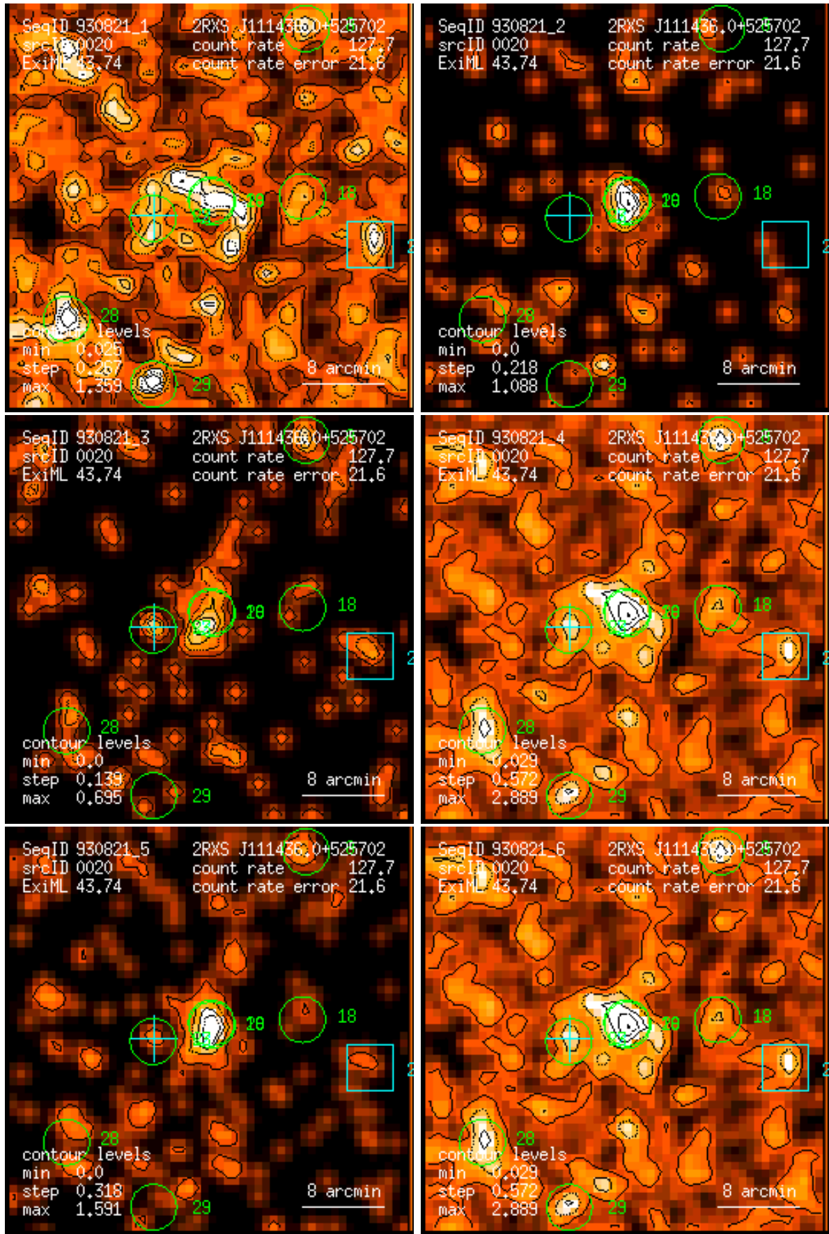
Figure 20: RASS 930821: detection 0020: band rate images, Gaussian filter: (1) PSPC channels 11 – 41, (2) 52 – 90, (3) 91 – 201, (4) 11 – 235, (5) 52 – 201, (6) 11 – 201. Broad band rates in counts/ks. Band rate contour levels in counts/ks/arcmin 2 .
