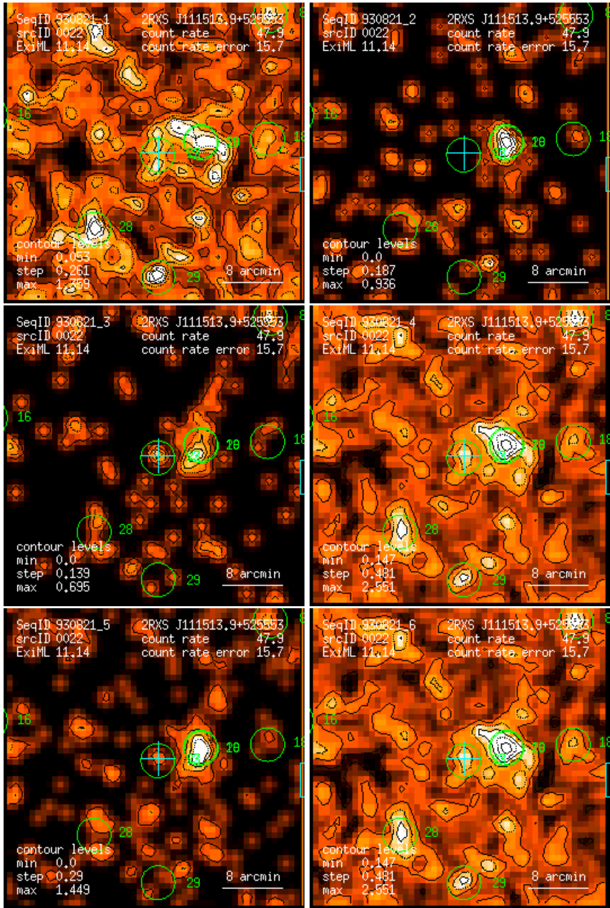
Figure 22: RASS 930821: detection 0022: band rate images, Gaussian filter: (1) PSPC channels 11 – 41, (2) 52 – 90, (3) 91 – 201, (4) 11 – 235, (5) 52 – 201, (6) 11 – 201. Broad band rates in counts/ks. Band rate contour levels in counts/ks/arcmin 2 .
