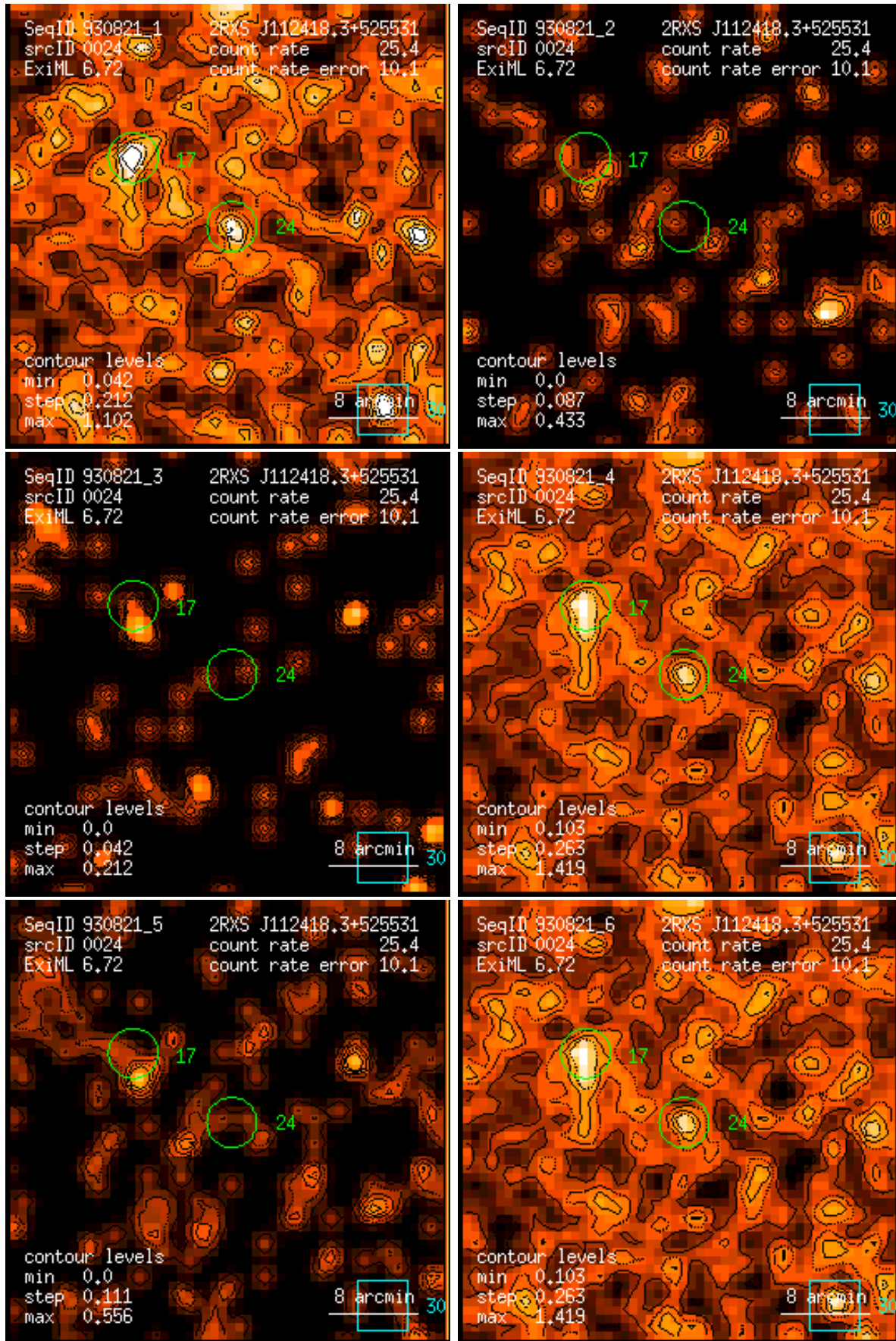
Figure 24: RASS 930821: detection 0024: band rate images, Gaussian filter: (1) PSPC channels 11 – 41, (2) 52 – 90, (3) 91 – 201, (4) 11 – 235, (5) 52 – 201, (6) 11 – 201. Broad band rates in counts/ks. Band rate contour levels in counts/ks/arcmin 2 .
