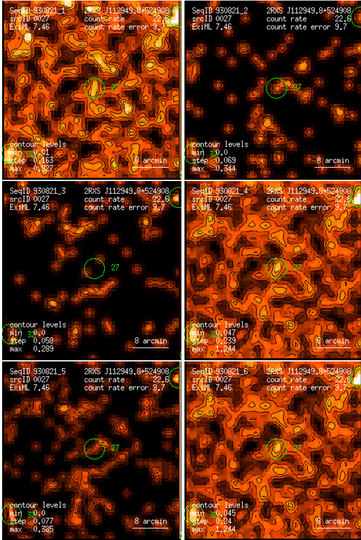
Figure 27: RASS 930821: detection 0027: band rate images, Gaussian filter: (1) PSPC channels 11 – 41, (2) 52 – 90, (3) 91 – 201, (4) 11 – 235, (5) 52 – 201, (6) 11 – 201. Broad band rates in counts/ks. Band rate contour levels in counts/ks/arcmin 2 .
