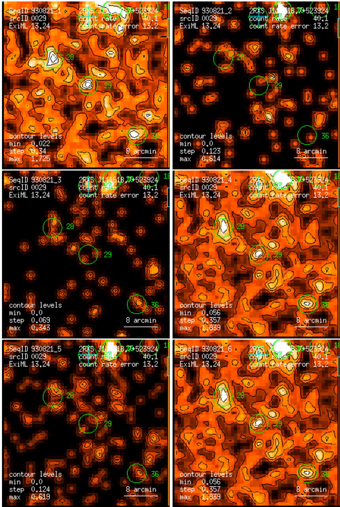
Figure 29: RASS 930821: detection 0029: band rate images, Gaussian filter: (1) PSPC channels 11 – 41, (2) 52 – 90, (3) 91 – 201, (4) 11 – 235, (5) 52 – 201, (6) 11 – 201. Broad band rates in counts/ks. Band rate contour levels in counts/ks/arcmin 2 .
