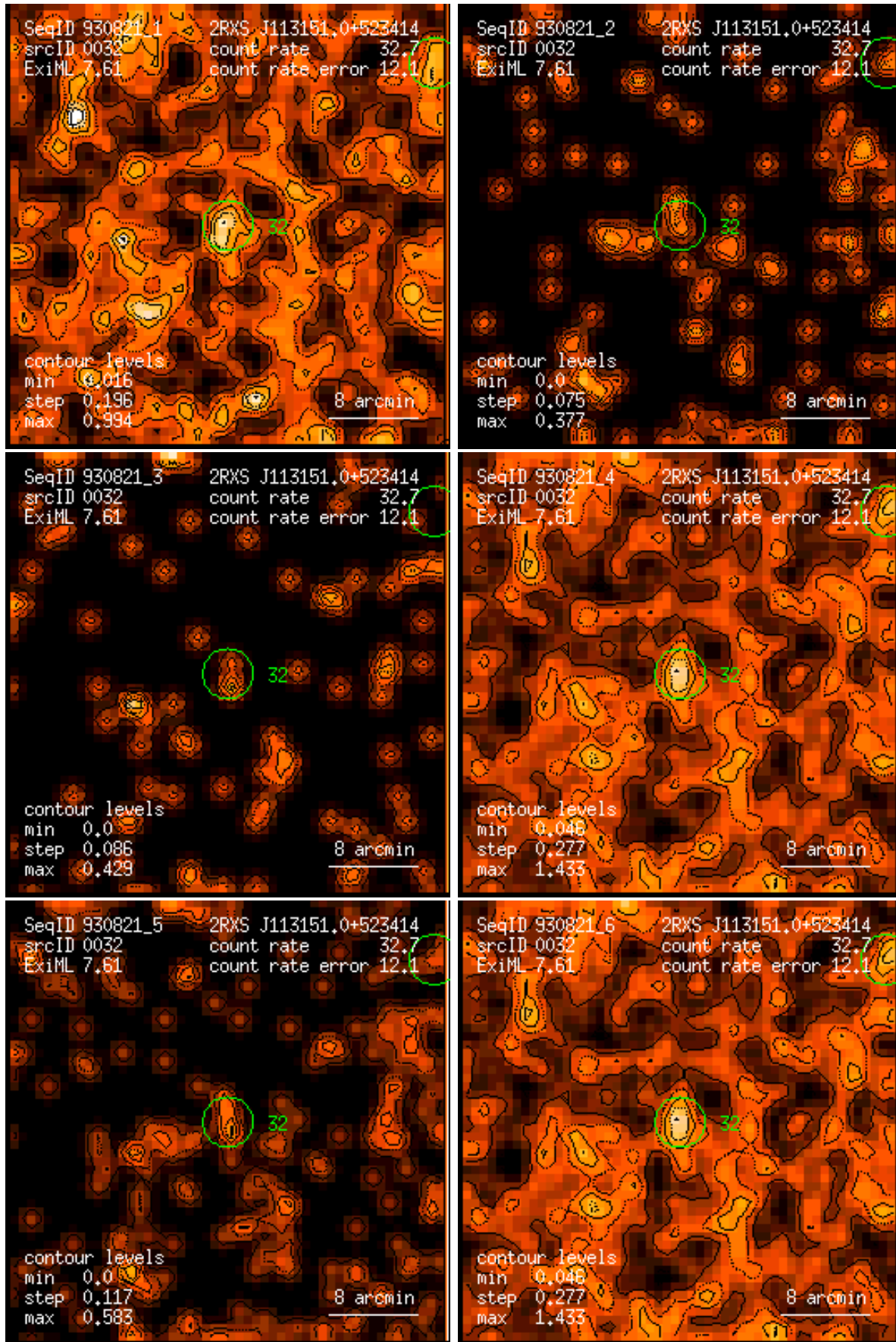
Figure 32: RASS 930821: detection 0032: band rate images, Gaussian filter: (1) PSPC channels 11 – 41, (2) 52 – 90, (3) 91 – 201, (4) 11 – 235, (5) 52 – 201, (6) 11 – 201. Broad band rates in counts/ks. Band rate contour levels in counts/ks/arcmin 2 .
