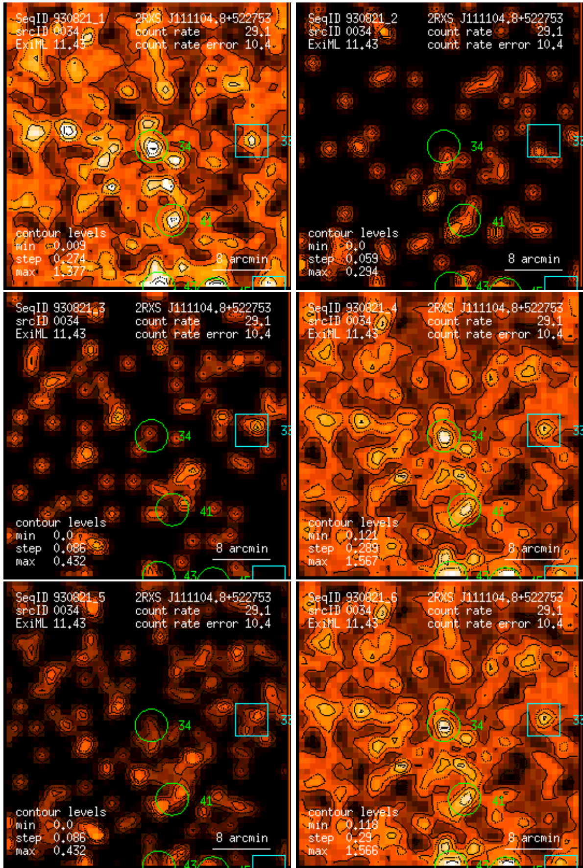
Figure 34: RASS 930821: detection 0034: band rate images, Gaussian filter: (1) PSPC channels 11 – 41, (2) 52 – 90, (3) 91 – 201, (4) 11 – 235, (5) 52 – 201, (6) 11 – 201. Broad band rates in counts/ks. Band rate contour levels in counts/ks/arcmin 2 .
