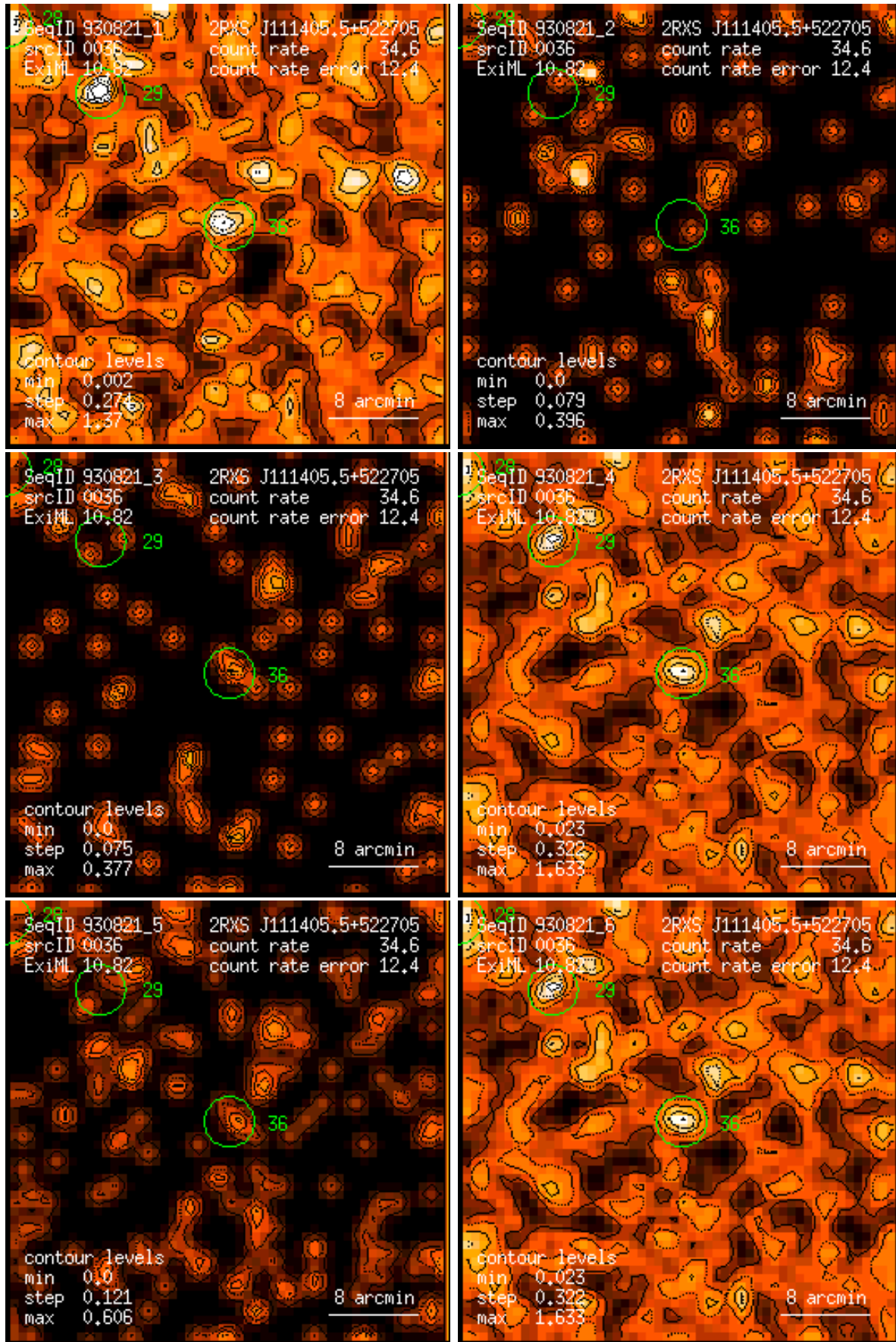
Figure 36: RASS 930821: detection 0036: band rate images, Gaussian filter: (1) PSPC channels 11 – 41, (2) 52 – 90, (3) 91 – 201, (4) 11 – 235, (5) 52 – 201, (6) 11 – 201. Broad band rates in counts/ks. Band rate contour levels in counts/ks/arcmin 2 .
