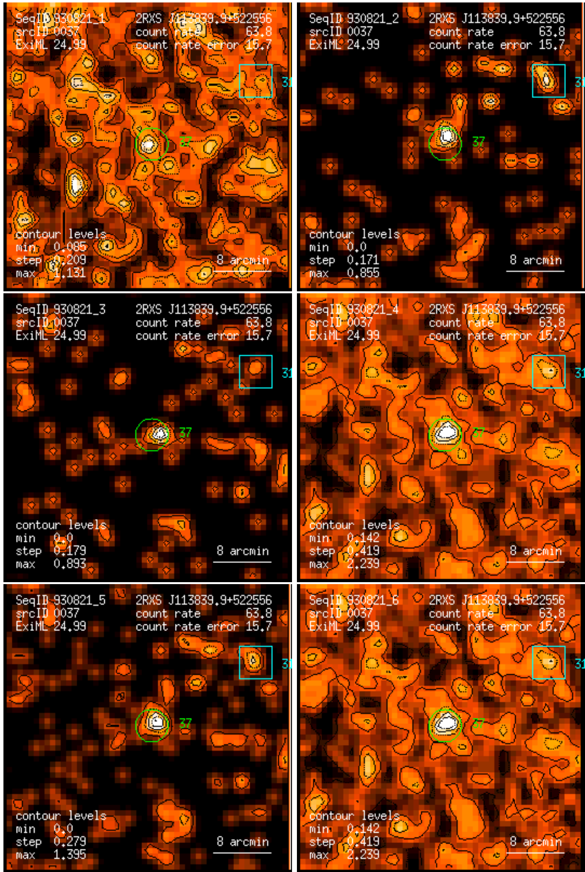
Figure 37: RASS 930821: detection 0037: band rate images, Gaussian filter: (1) PSPC channels 11 – 41, (2) 52 – 90, (3) 91 – 201, (4) 11 – 235, (5) 52 – 201, (6) 11 – 201. Broad band rates in counts/ks. Band rate contour levels in counts/ks/arcmin 2 .
