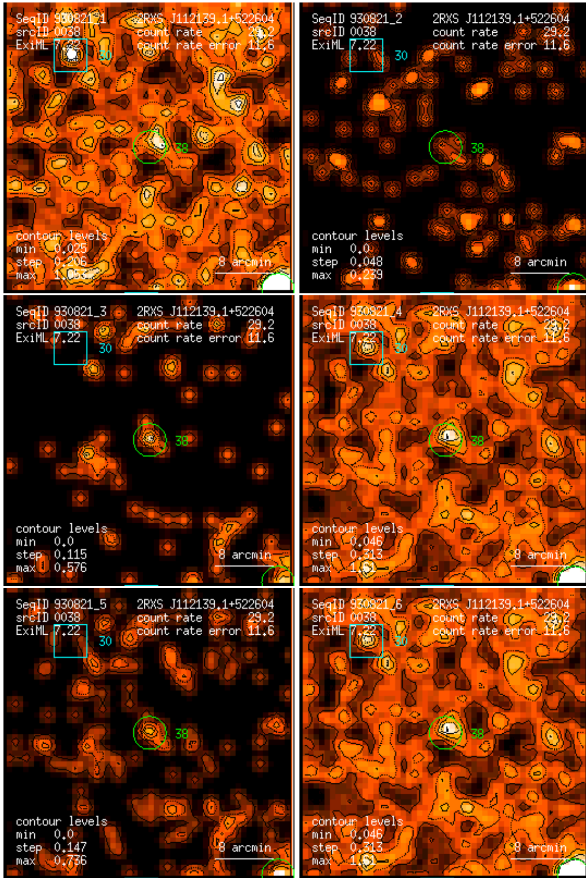
Figure 38: RASS 930821: detection 0038: band rate images, Gaussian filter: (1) PSPC channels 11 – 41, (2) 52 – 90, (3) 91 – 201, (4) 11 – 235, (5) 52 – 201, (6) 11 – 201. Broad band rates in counts/ks. Band rate contour levels in counts/ks/arcmin 2 .
