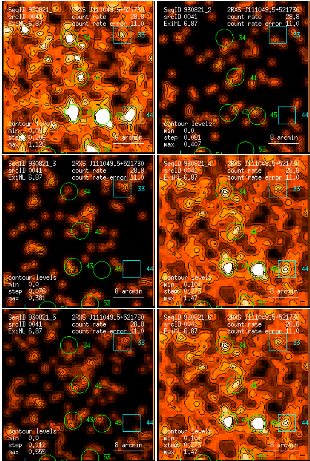
Figure 41: RASS 930821: detection 0041: band rate images, Gaussian filter: (1) PSPC channels 11 – 41, (2) 52 – 90, (3) 91 – 201, (4) 11 – 235, (5) 52 – 201, (6) 11 – 201. Broad band rates in counts/ks. Band rate contour levels in counts/ks/arcmin 2 .
