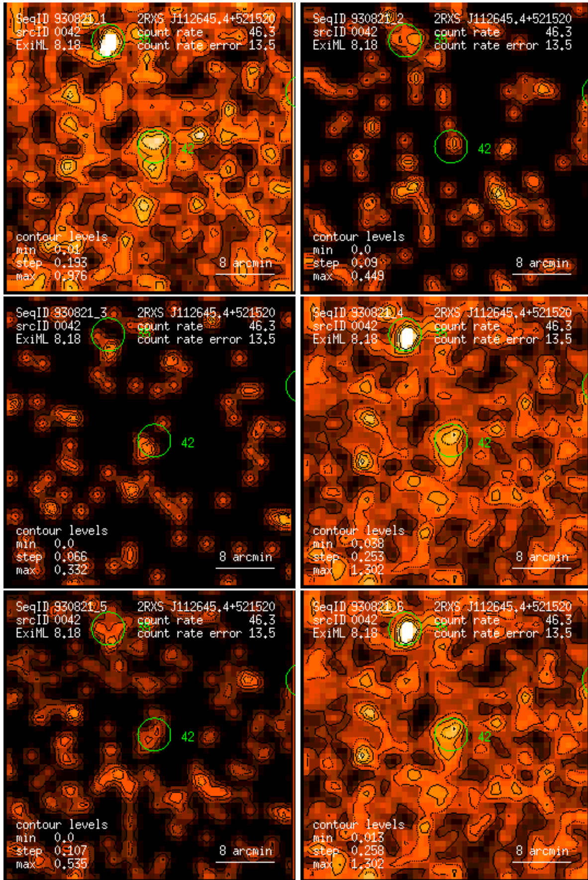
Figure 42: RASS 930821: detection 0042: band rate images, Gaussian filter: (1) PSPC channels 11 – 41, (2) 52 – 90, (3) 91 – 201, (4) 11 – 235, (5) 52 – 201, (6) 11 – 201. Broad band rates in counts/ks. Band rate contour levels in counts/ks/arcmin 2 .
