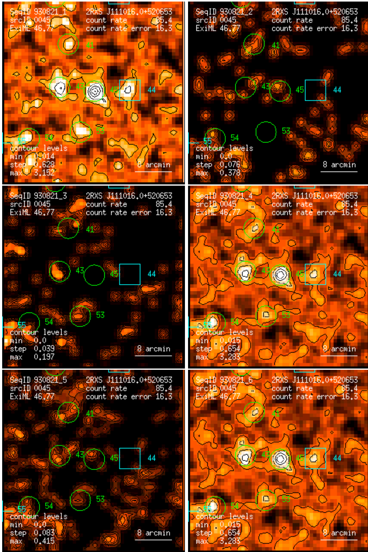
Figure 45: RASS 930821: detection 0045: band rate images, Gaussian filter: (1) PSPC channels 11 – 41, (2) 52 – 90, (3) 91 – 201, (4) 11 – 235, (5) 52 – 201, (6) 11 – 201. Broad band rates in counts/ks. Band rate contour levels in counts/ks/arcmin 2 .
