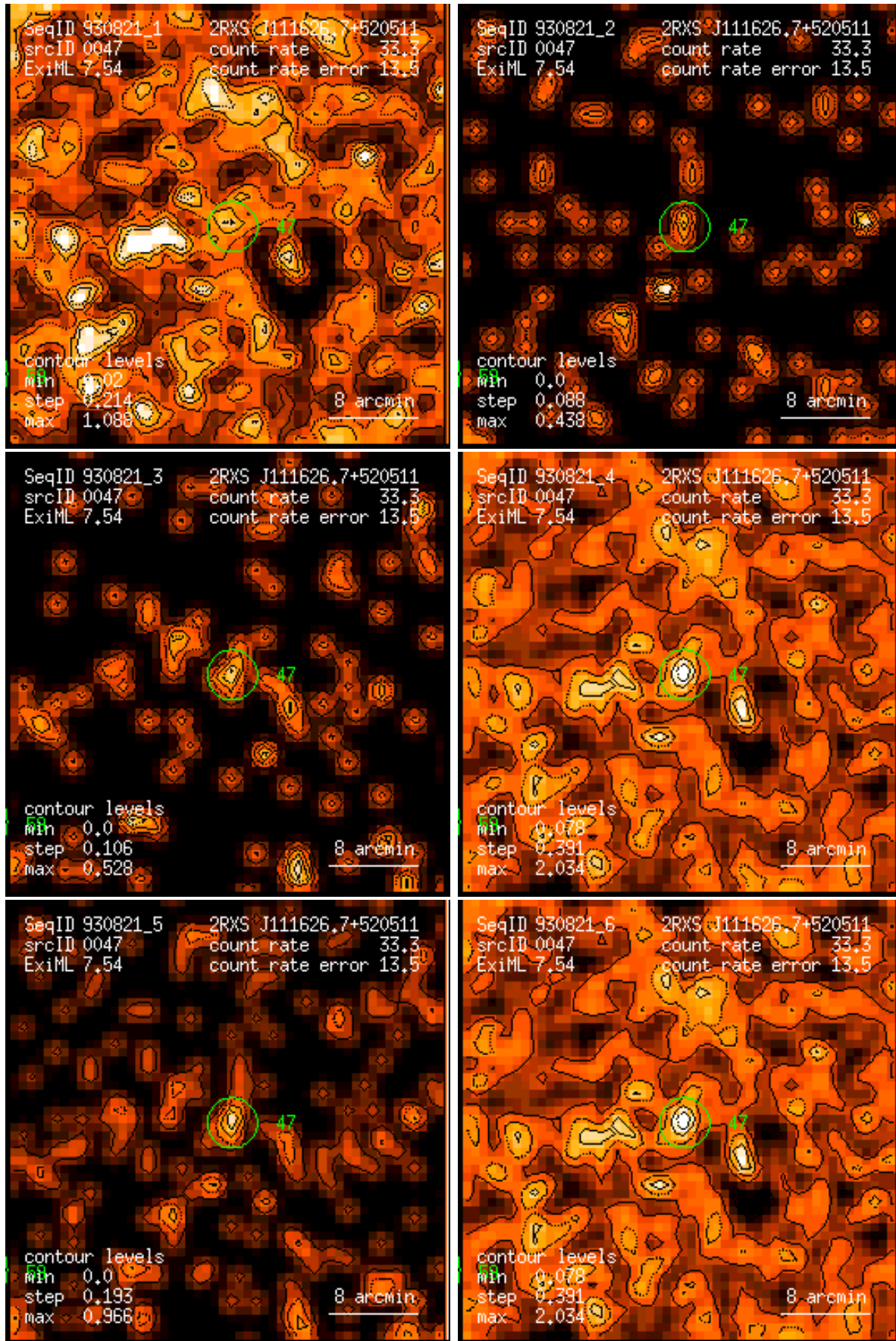
Figure 47: RASS 930821: detection 0047: band rate images, Gaussian filter: (1) PSPC channels 11 – 41, (2) 52 – 90, (3) 91 – 201, (4) 11 – 235, (5) 52 – 201, (6) 11 – 201. Broad band rates in counts/ks. Band rate contour levels in counts/ks/arcmin 2 .
