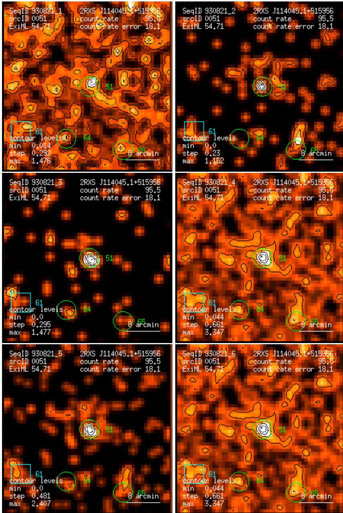
Figure 51: RASS 930821: detection 0051: band rate images, Gaussian filter: (1) PSPC channels 11 – 41, (2) 52 – 90, (3) 91 – 201, (4) 11 – 235, (5) 52 – 201, (6) 11 – 201. Broad band rates in counts/ks. Band rate contour levels in counts/ks/arcmin 2 .
