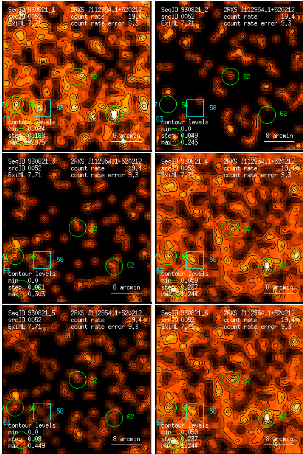
Figure 52: RASS 930821: detection 0052: band rate images, Gaussian filter: (1) PSPC channels 11 – 41, (2) 52 – 90, (3) 91 – 201, (4) 11 – 235, (5) 52 – 201, (6) 11 – 201. Broad band rates in counts/ks. Band rate contour levels in counts/ks/arcmin 2 .
