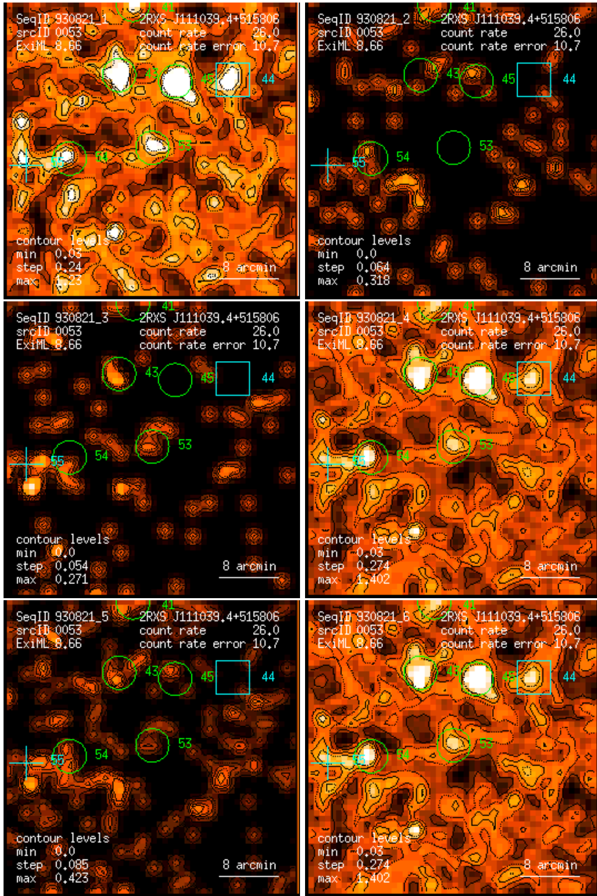
Figure 53: RASS 930821: detection 0053: band rate images, Gaussian filter: (1) PSPC channels 11 – 41, (2) 52 – 90, (3) 91 – 201, (4) 11 – 235, (5) 52 – 201, (6) 11 – 201. Broad band rates in counts/ks. Band rate contour levels in counts/ks/arcmin 2 .
