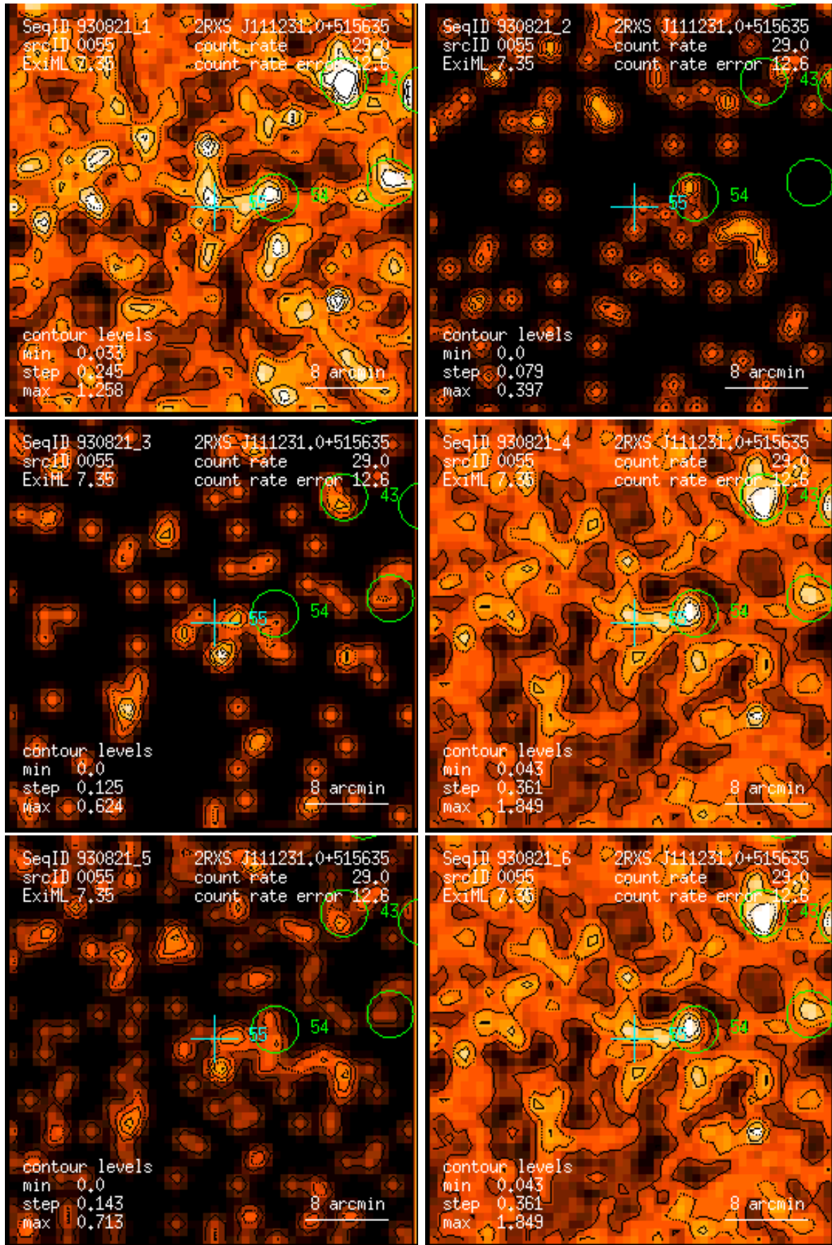
Figure 55: RASS 930821: detection 0055: band rate images, Gaussian filter: (1) PSPC channels 11 – 41, (2) 52 – 90, (3) 91 – 201, (4) 11 – 235, (5) 52 – 201, (6) 11 – 201. Broad band rates in counts/ks. Band rate contour levels in counts/ks/arcmin 2 .
