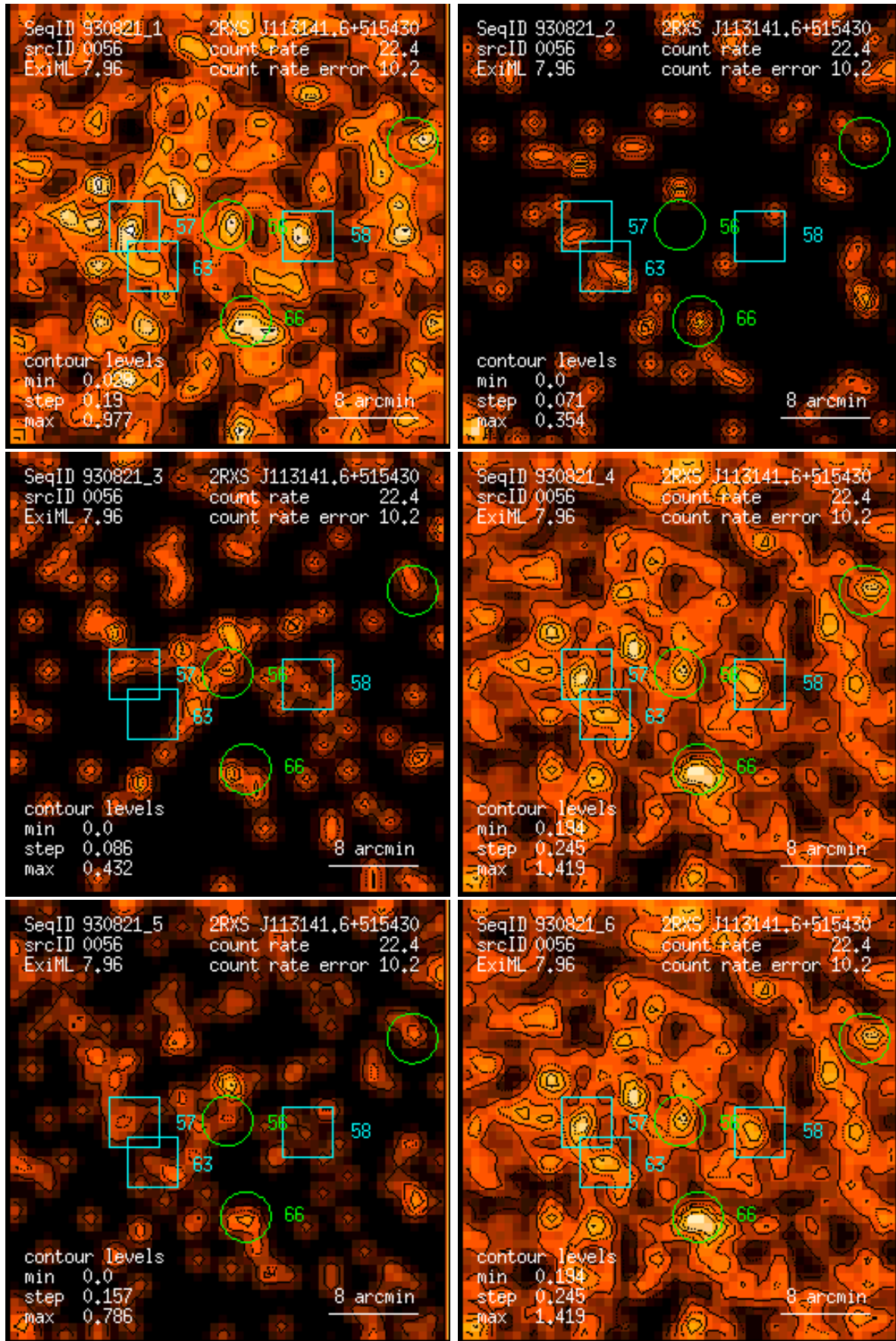
Figure 56: RASS 930821: detection 0056: band rate images, Gaussian filter: (1) PSPC channels 11 – 41, (2) 52 – 90, (3) 91 – 201, (4) 11 – 235, (5) 52 – 201, (6) 11 – 201. Broad band rates in counts/ks. Band rate contour levels in counts/ks/arcmin 2 .
