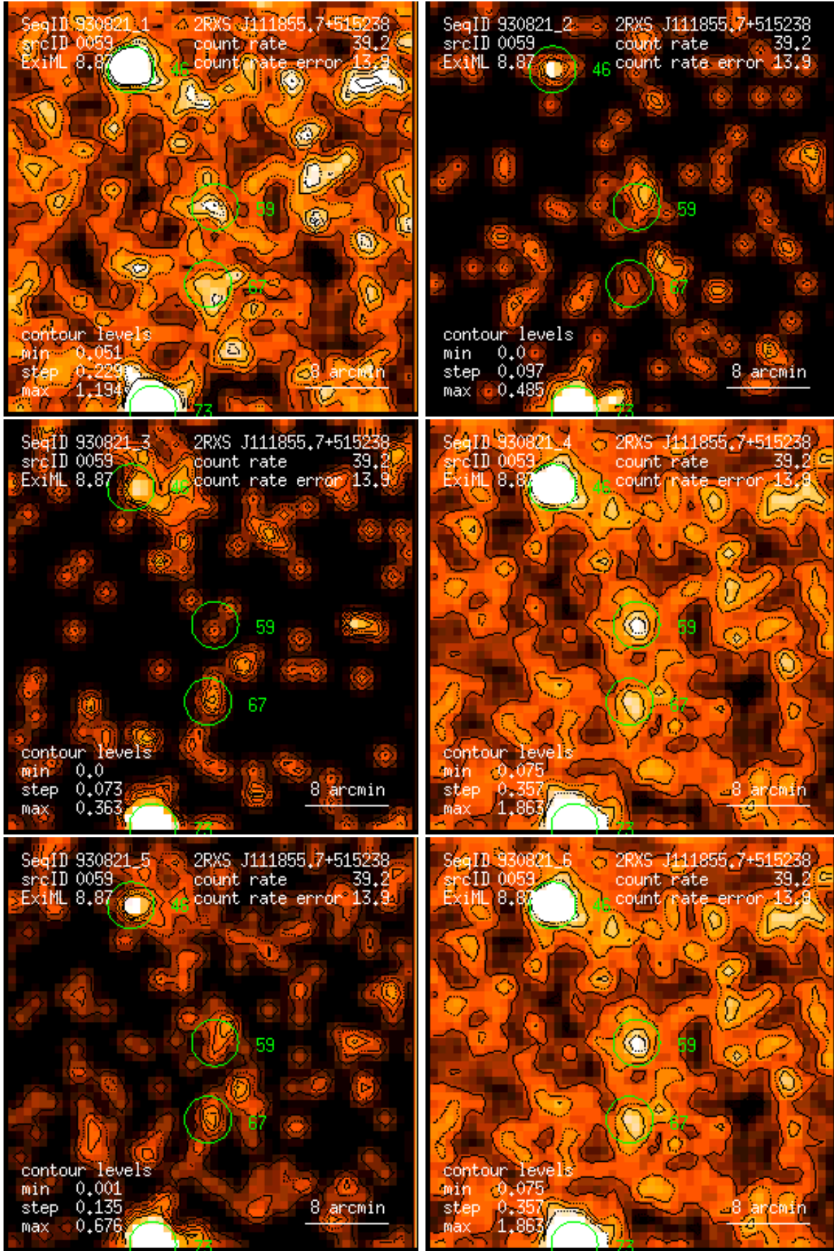
Figure 59: RASS 930821: detection 0059: band rate images, Gaussian filter: (1) PSPC channels 11 – 41, (2) 52 – 90, (3) 91 – 201, (4) 11 – 235, (5) 52 – 201, (6) 11 – 201. Broad band rates in counts/ks. Band rate contour levels in counts/ks/arcmin 2 .
