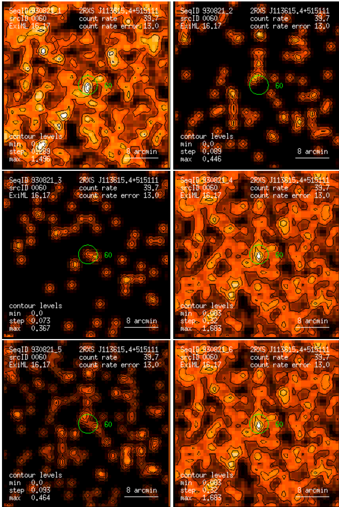
Figure 60: RASS 930821: detection 0060: band rate images, Gaussian filter: (1) PSPC channels 11 – 41, (2) 52 – 90, (3) 91 – 201, (4) 11 – 235, (5) 52 – 201, (6) 11 – 201. Broad band rates in counts/ks. Band rate contour levels in counts/ks/arcmin 2 .
