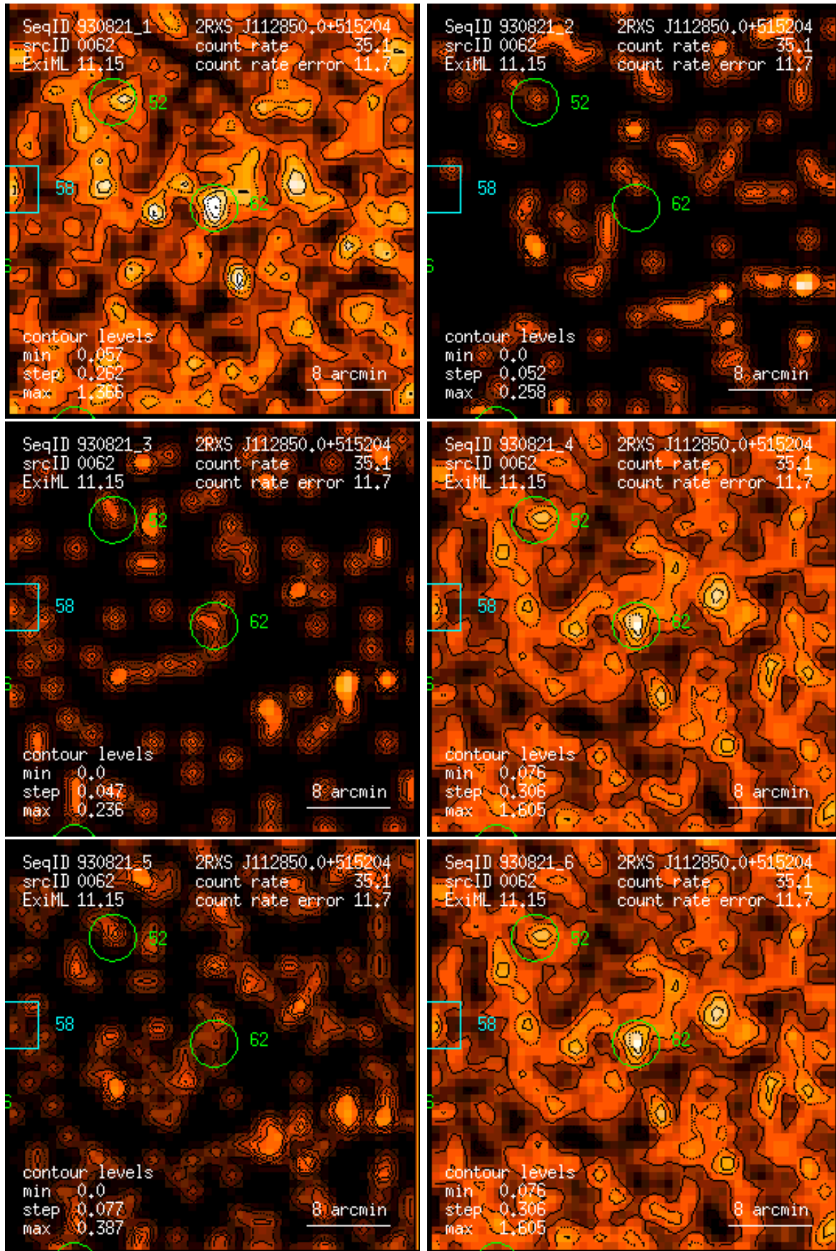
Figure 62: RASS 930821: detection 0062: band rate images, Gaussian filter: (1) PSPC channels 11 – 41, (2) 52 – 90, (3) 91 – 201, (4) 11 – 235, (5) 52 – 201, (6) 11 – 201. Broad band rates in counts/ks. Band rate contour levels in counts/ks/arcmin 2 .
