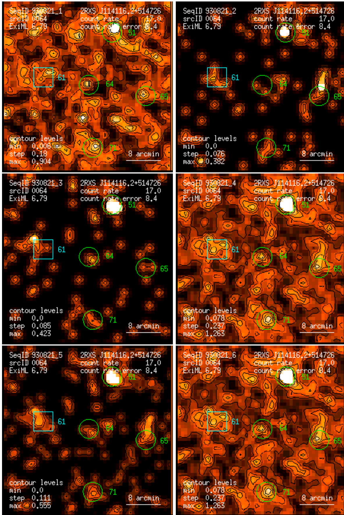
Figure 64: RASS 930821: detection 0064: band rate images, Gaussian filter: (1) PSPC channels 11 – 41, (2) 52 – 90, (3) 91 – 201, (4) 11 – 235, (5) 52 – 201, (6) 11 – 201. Broad band rates in counts/ks. Band rate contour levels in counts/ks/arcmin 2 .
