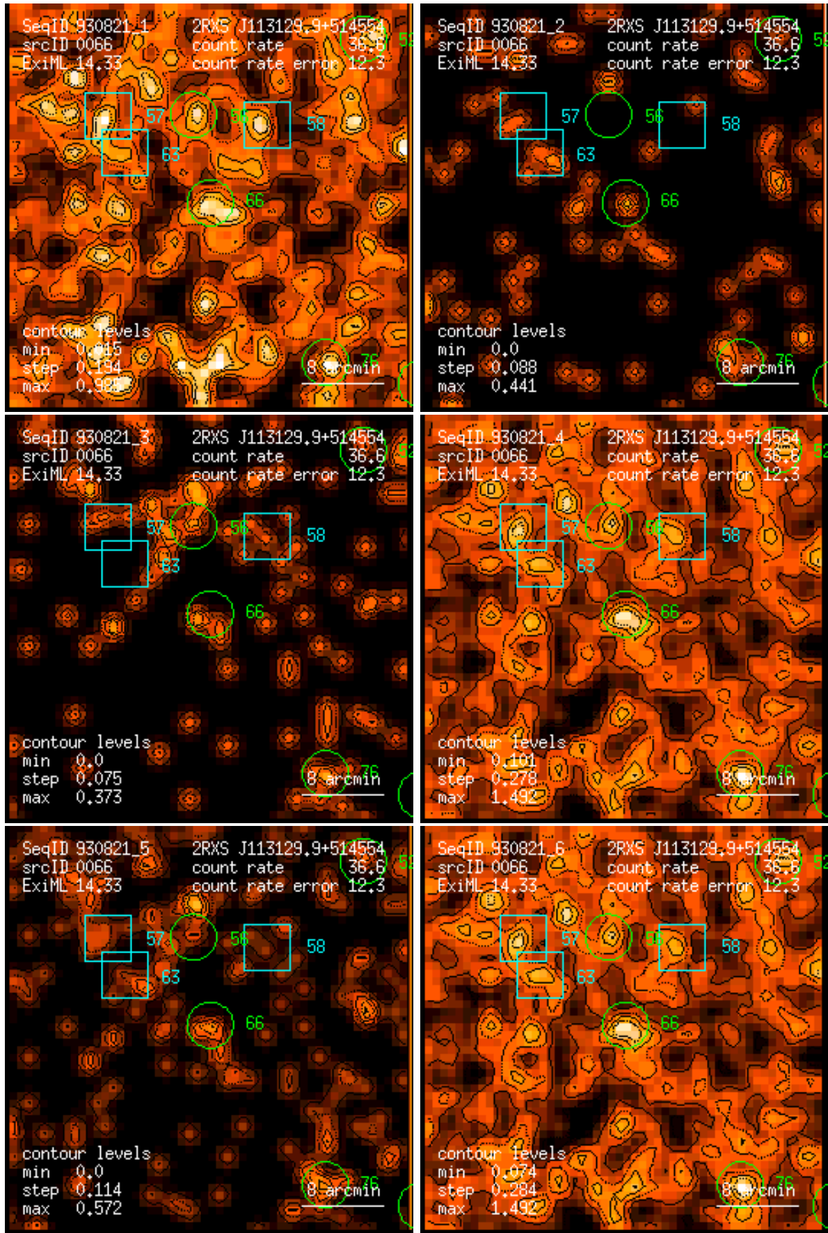
Figure 66: RASS 930821: detection 0066: band rate images, Gaussian filter: (1) PSPC channels 11 – 41, (2) 52 – 90, (3) 91 – 201, (4) 11 – 235, (5) 52 – 201, (6) 11 – 201. Broad band rates in counts/ks. Band rate contour levels in counts/ks/arcmin 2 .
