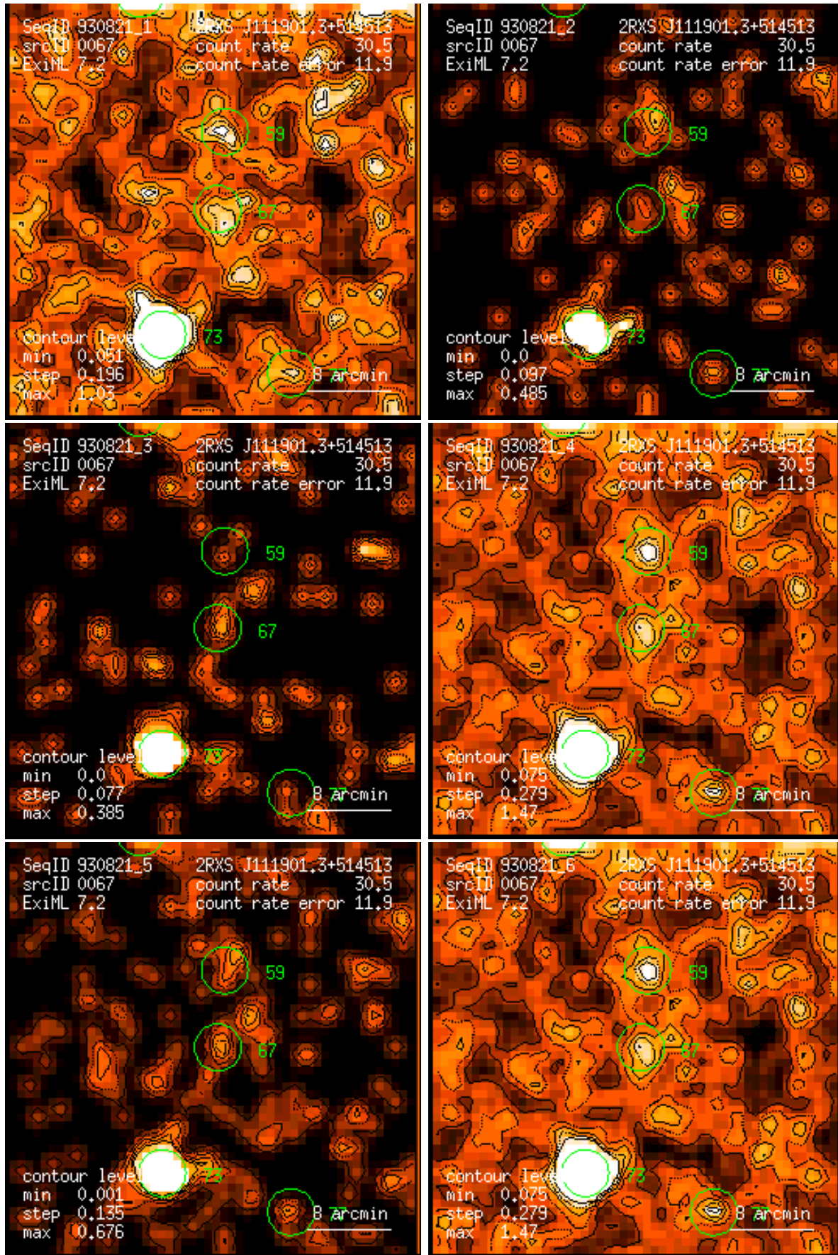
Figure 67: RASS 930821: detection 0067: band rate images, Gaussian filter: (1) PSPC channels 11 – 41, (2) 52 – 90, (3) 91 – 201, (4) 11 – 235, (5) 52 – 201, (6) 11 – 201. Broad band rates in counts/ks. Band rate contour levels in counts/ks/arcmin 2 .
