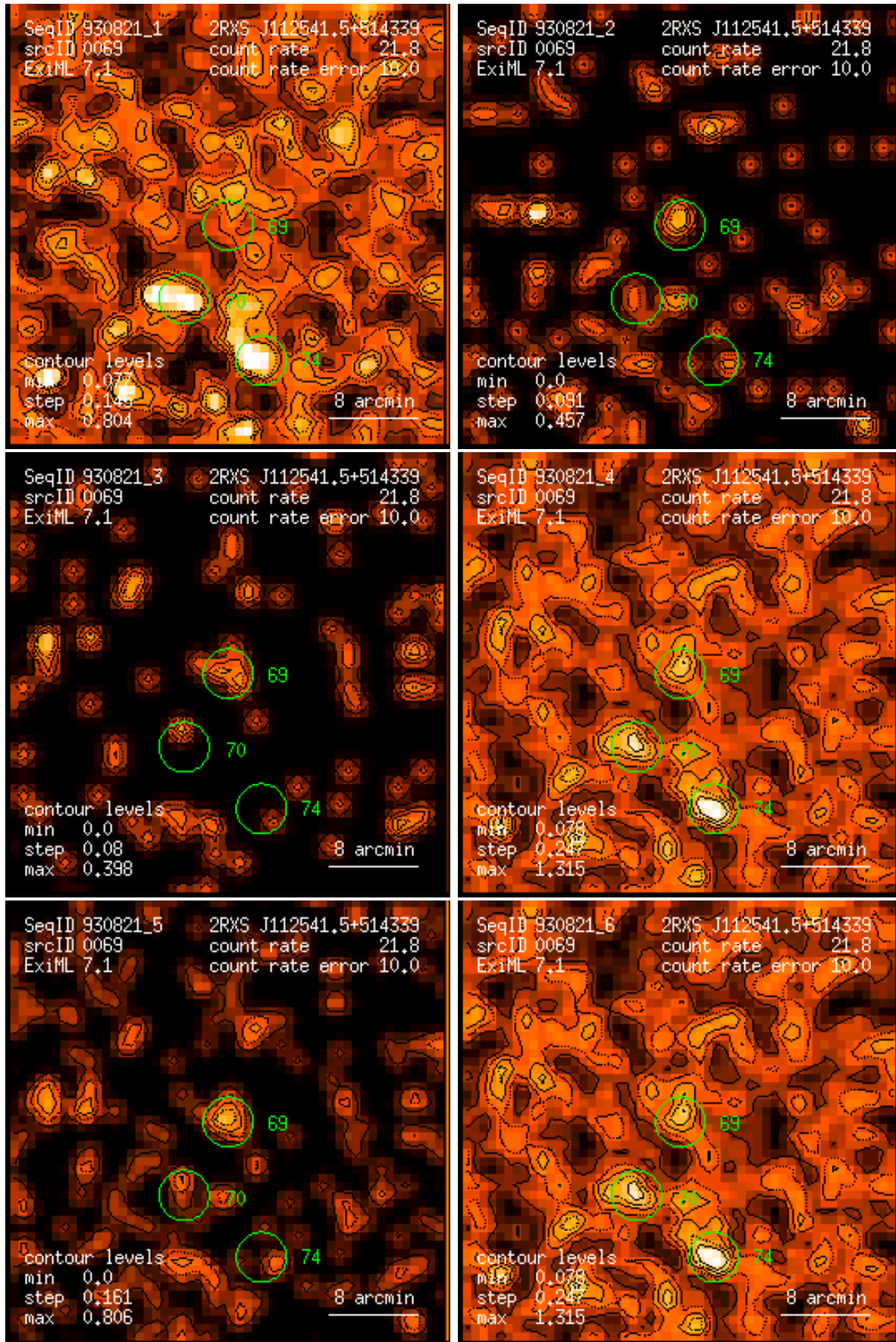
Figure 69: RASS 930821: detection 0069: band rate images, Gaussian filter: (1) PSPC channels 11 – 41, (2) 52 – 90, (3) 91 – 201, (4) 11 – 235, (5) 52 – 201, (6) 11 – 201. Broad band rates in counts/ks. Band rate contour levels in counts/ks/arcmin 2 .
