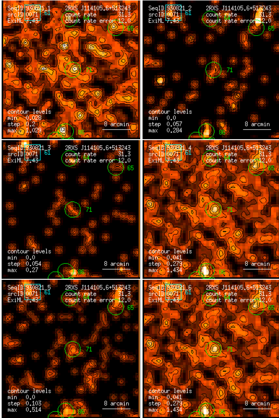
Figure 71: RASS 930821: detection 0071: band rate images, Gaussian filter: (1) PSPC channels 11 – 41, (2) 52 – 90, (3) 91 – 201, (4) 11 – 235, (5) 52 – 201, (6) 11 – 201. Broad band rates in counts/ks. Band rate contour levels in counts/ks/arcmin 2 .
