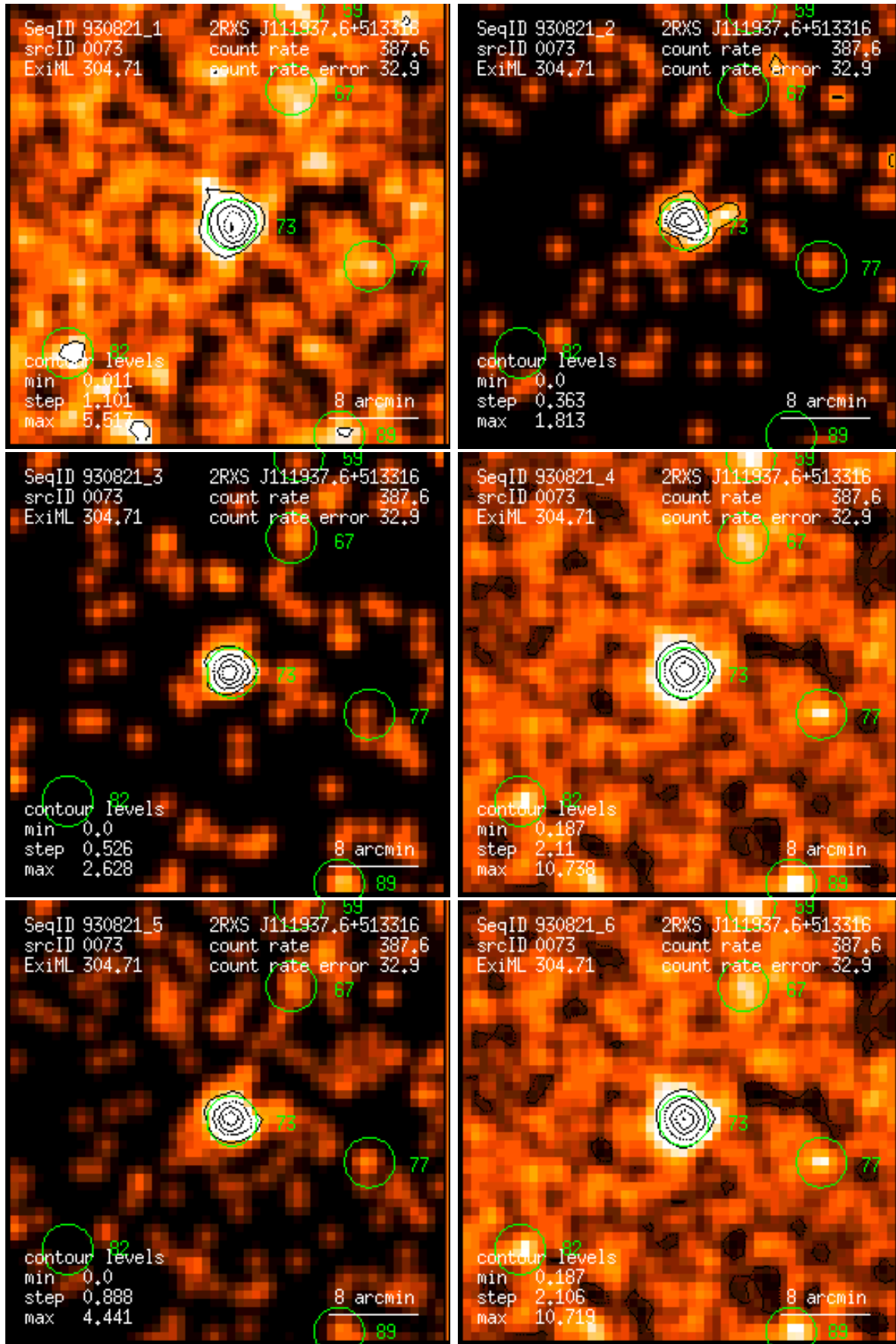
Figure 73: RASS 930821: detection 0073: band rate images, Gaussian filter: (1) PSPC channels 11 – 41, (2) 52 – 90, (3) 91 – 201, (4) 11 – 235, (5) 52 – 201, (6) 11 – 201. Broad band rates in counts/ks. Band rate contour levels in counts/ks/arcmin 2 .
