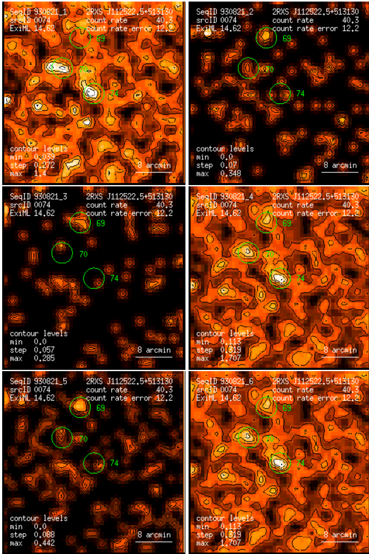
Figure 74: RASS 930821: detection 0074: band rate images, Gaussian filter: (1) PSPC channels 11 – 41, (2) 52 – 90, (3) 91 – 201, (4) 11 – 235, (5) 52 – 201, (6) 11 – 201. Broad band rates in counts/ks. Band rate contour levels in counts/ks/arcmin 2 .
