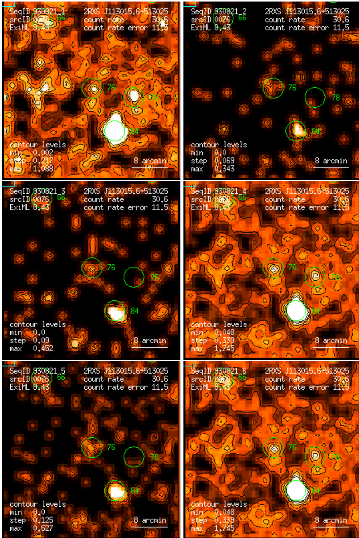
Figure 76: RASS 930821: detection 0076: band rate images, Gaussian filter: (1) PSPC channels 11 – 41, (2) 52 – 90, (3) 91 – 201, (4) 11 – 235, (5) 52 – 201, (6) 11 – 201. Broad band rates in counts/ks. Band rate contour levels in counts/ks/arcmin 2 .
