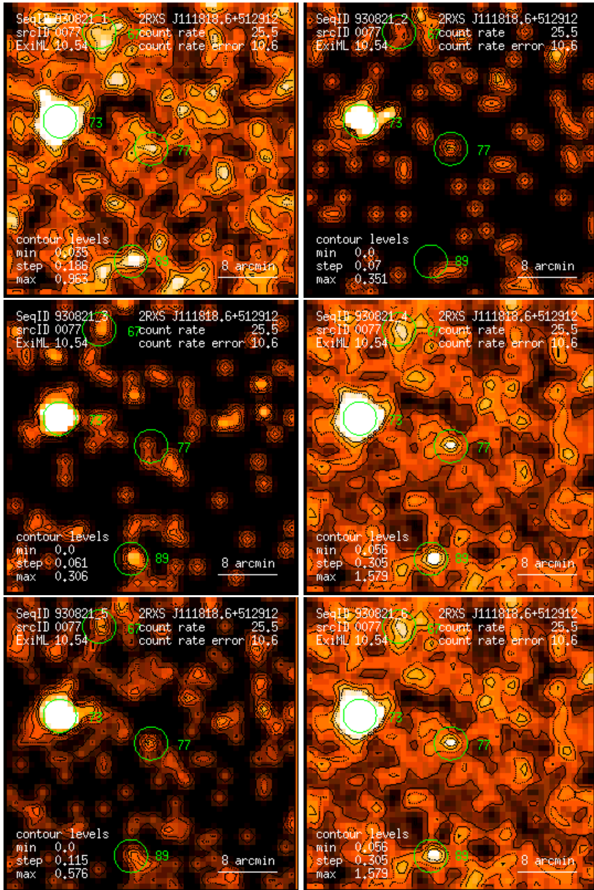
Figure 77: RASS 930821: detection 0077: band rate images, Gaussian filter: (1) PSPC channels 11 – 41, (2) 52 – 90, (3) 91 – 201, (4) 11 – 235, (5) 52 – 201, (6) 11 – 201. Broad band rates in counts/ks. Band rate contour levels in counts/ks/arcmin 2 .
