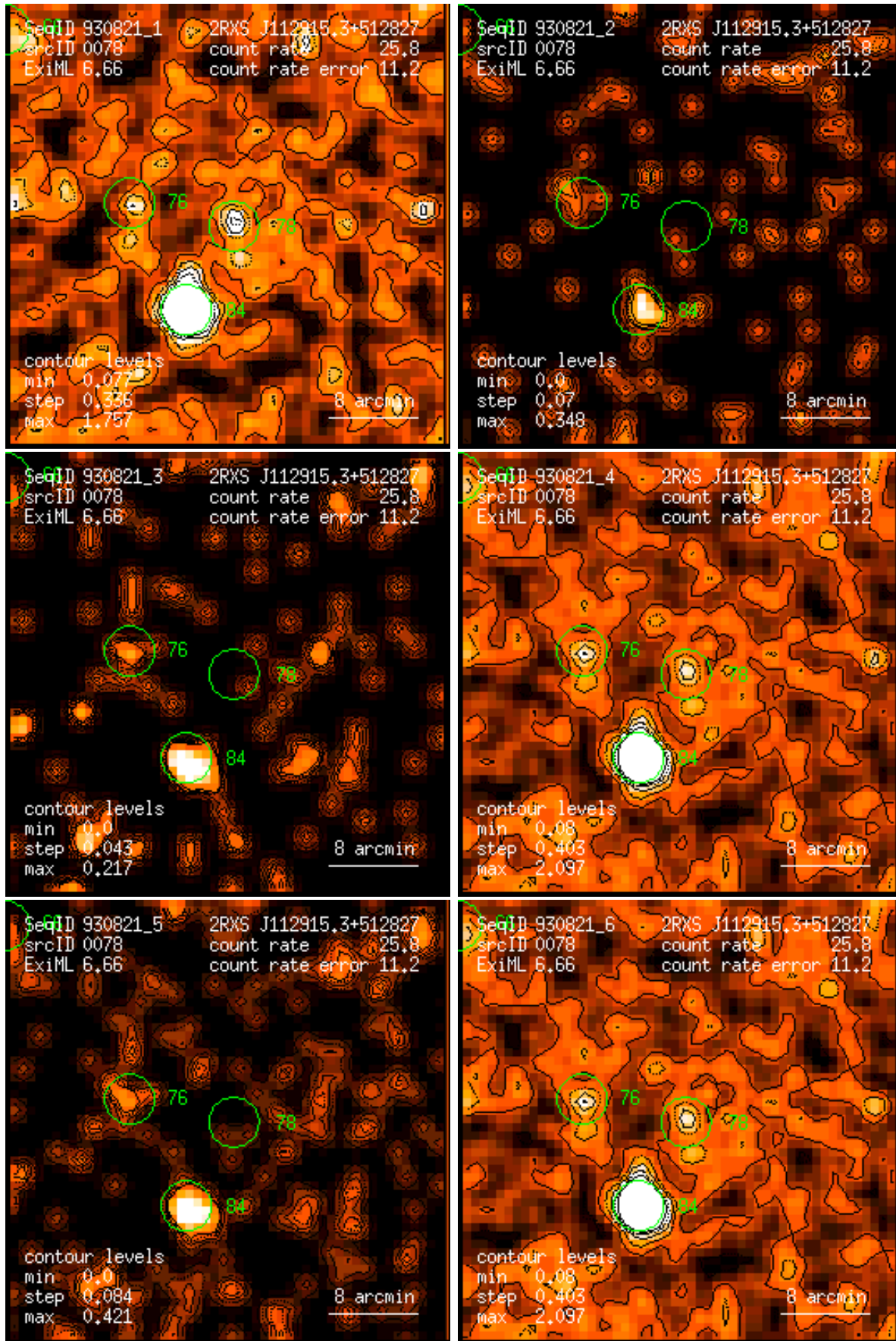
Figure 78: RASS 930821: detection 0078: band rate images, Gaussian filter: (1) PSPC channels 11 – 41, (2) 52 – 90, (3) 91 – 201, (4) 11 – 235, (5) 52 – 201, (6) 11 – 201. Broad band rates in counts/ks. Band rate contour levels in counts/ks/arcmin 2 .
