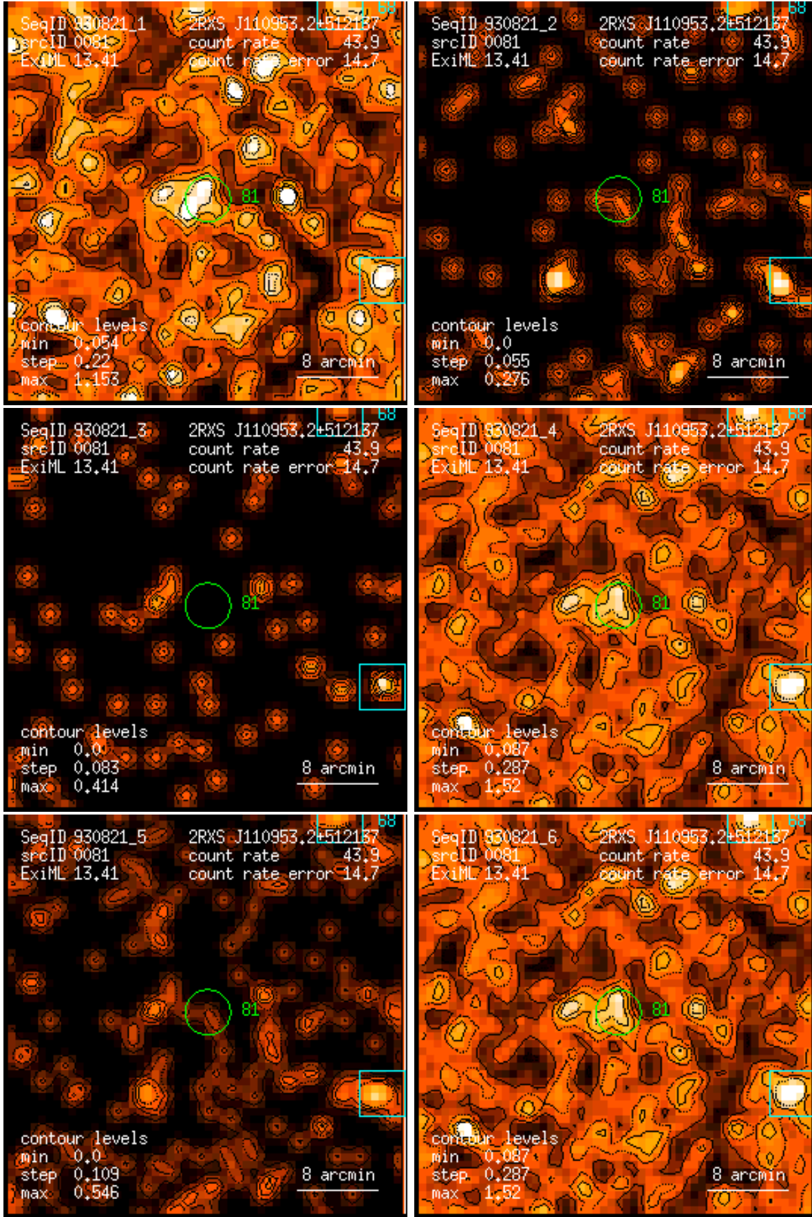
Figure 81: RASS 930821: detection 0081: band rate images, Gaussian filter: (1) PSPC channels 11 – 41, (2) 52 – 90, (3) 91 – 201, (4) 11 – 235, (5) 52 – 201, (6) 11 – 201. Broad band rates in counts/ks. Band rate contour levels in counts/ks/arcmin 2 .
