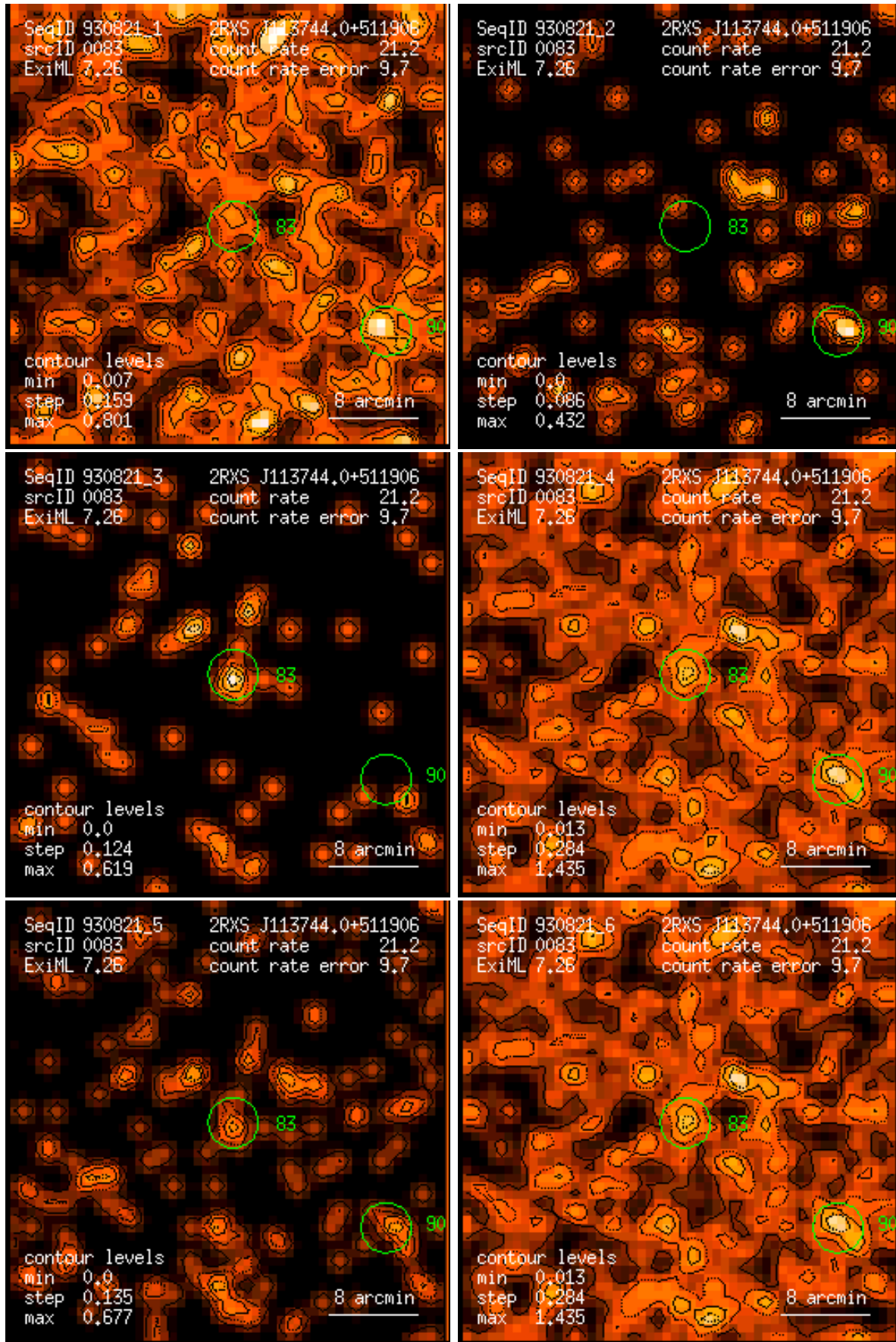
Figure 83: RASS 930821: detection 0083: band rate images, Gaussian filter: (1) PSPC channels 11 – 41, (2) 52 – 90, (3) 91 – 201, (4) 11 – 235, (5) 52 – 201, (6) 11 – 201. Broad band rates in counts/ks. Band rate contour levels in counts/ks/arcmin 2 .
