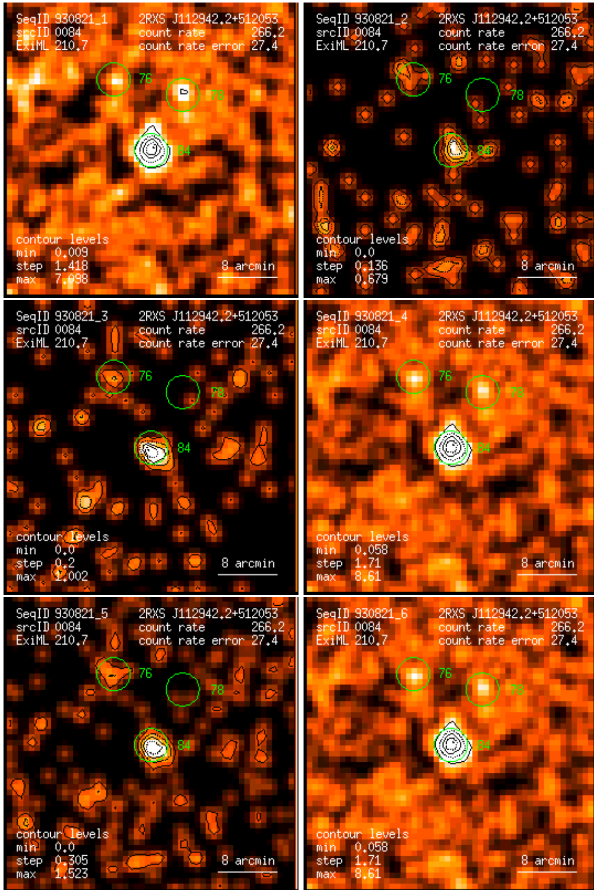
Figure 84: RASS 930821: detection 0084: band rate images, Gaussian filter: (1) PSPC channels 11 – 41, (2) 52 – 90, (3) 91 – 201, (4) 11 – 235, (5) 52 – 201, (6) 11 – 201. Broad band rates in counts/ks. Band rate contour levels in counts/ks/arcmin 2 .
