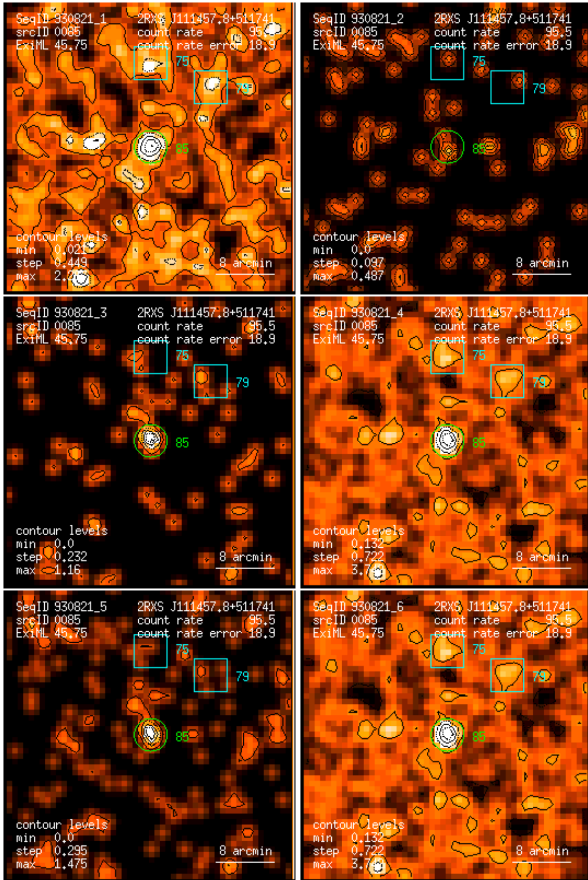
Figure 85: RASS 930821: detection 0085: band rate images, Gaussian filter: (1) PSPC channels 11 – 41, (2) 52 – 90, (3) 91 – 201, (4) 11 – 235, (5) 52 – 201, (6) 11 – 201. Broad band rates in counts/ks. Band rate contour levels in counts/ks/arcmin 2 .
