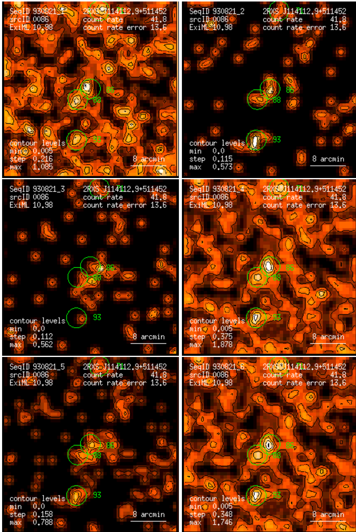
Figure 86: RASS 930821: detection 0086: band rate images, Gaussian filter: (1) PSPC channels 11 – 41, (2) 52 – 90, (3) 91 – 201, (4) 11 – 235, (5) 52 – 201, (6) 11 – 201. Broad band rates in counts/ks. Band rate contour levels in counts/ks/arcmin 2 .
