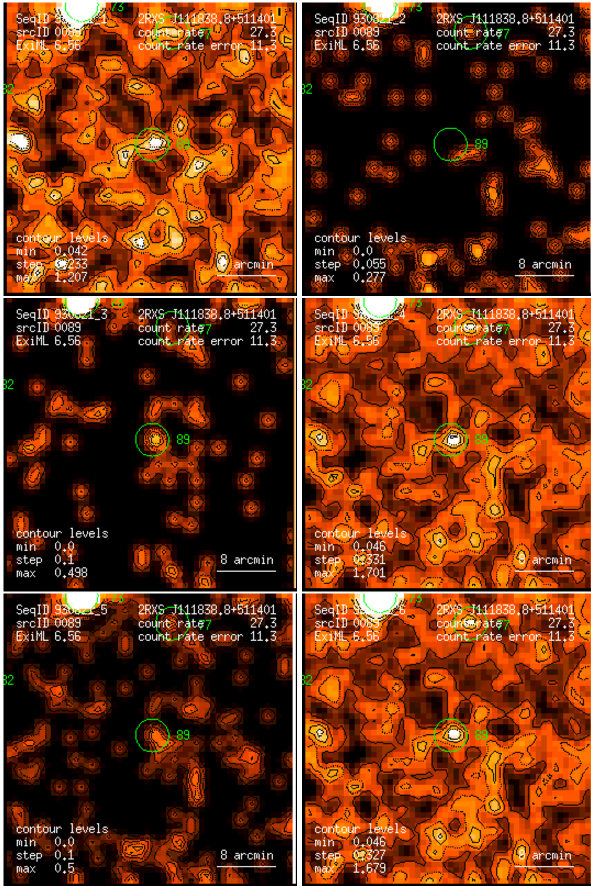
Figure 89: RASS 930821: detection 0089: band rate images, Gaussian filter: (1) PSPC channels 11 – 41, (2) 52 – 90, (3) 91 – 201, (4) 11 – 235, (5) 52 – 201, (6) 11 – 201. Broad band rates in counts/ks. Band rate contour levels in counts/ks/arcmin 2 .
