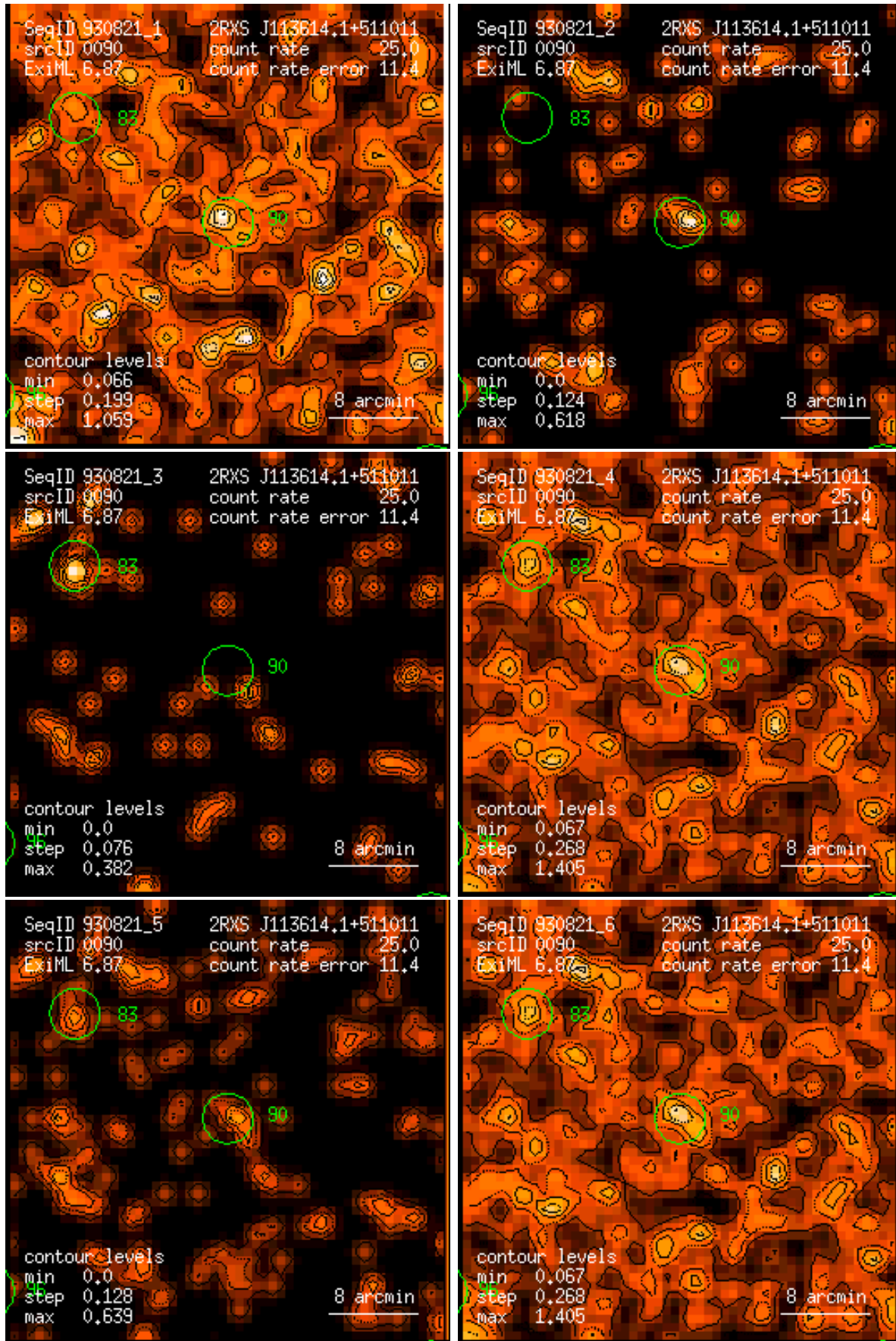
Figure 90: RASS 930821: detection 0090: band rate images, Gaussian filter: (1) PSPC channels 11 – 41, (2) 52 – 90, (3) 91 – 201, (4) 11 – 235, (5) 52 – 201, (6) 11 – 201. Broad band rates in counts/ks. Band rate contour levels in counts/ks/arcmin 2 .
