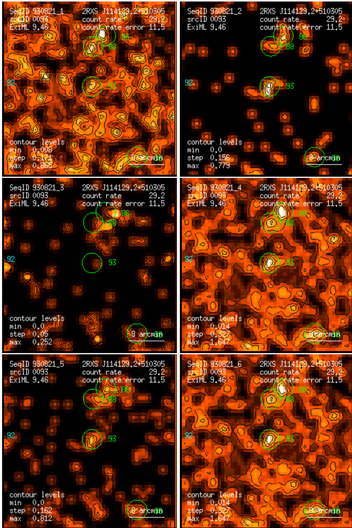
Figure 93: RASS 930821: detection 0093: band rate images, Gaussian filter: (1) PSPC channels 11 – 41, (2) 52 – 90, (3) 91 – 201, (4) 11 – 235, (5) 52 – 201, (6) 11 – 201. Broad band rates in counts/ks. Band rate contour levels in counts/ks/arcmin 2 .
